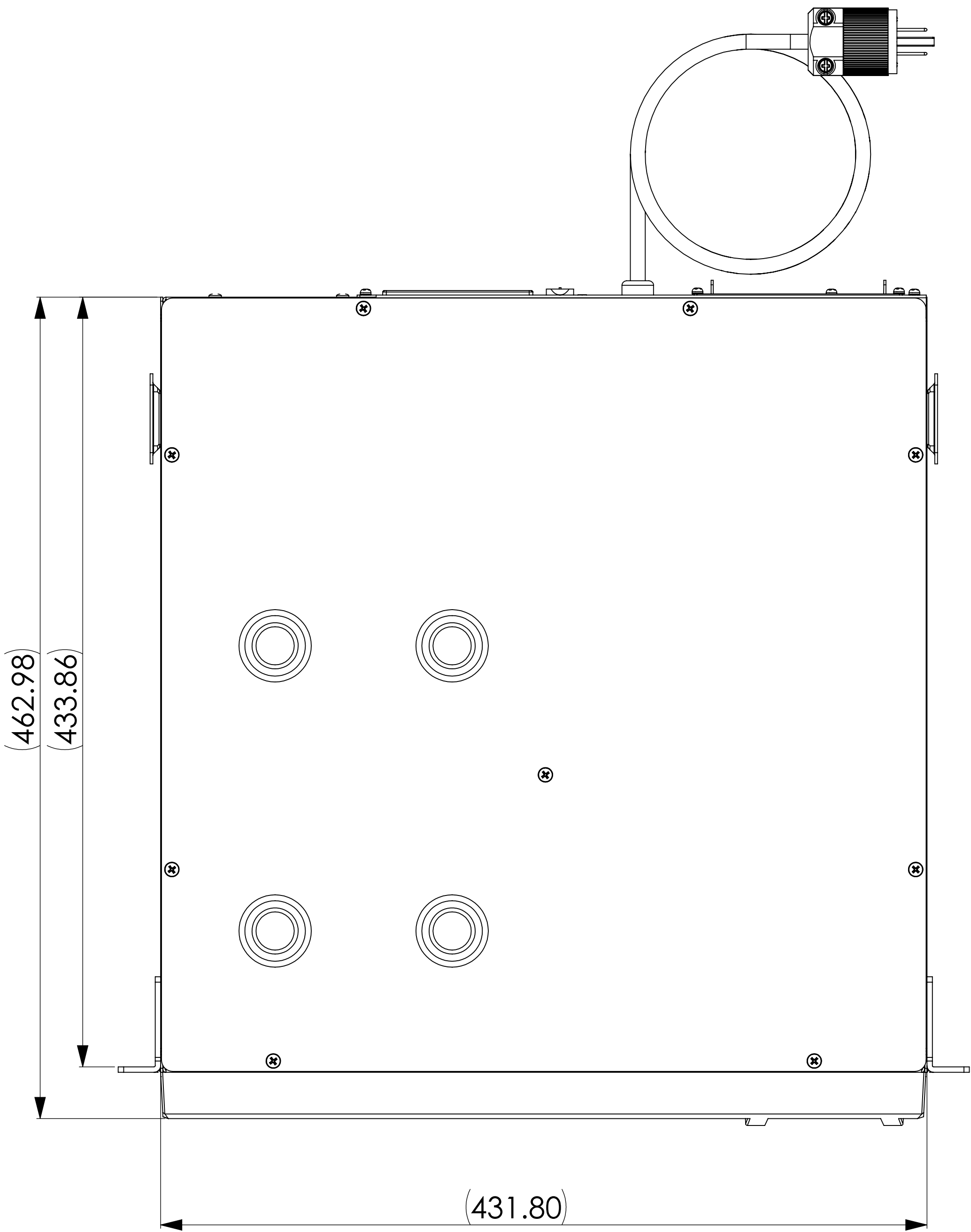
TOP VIEW
