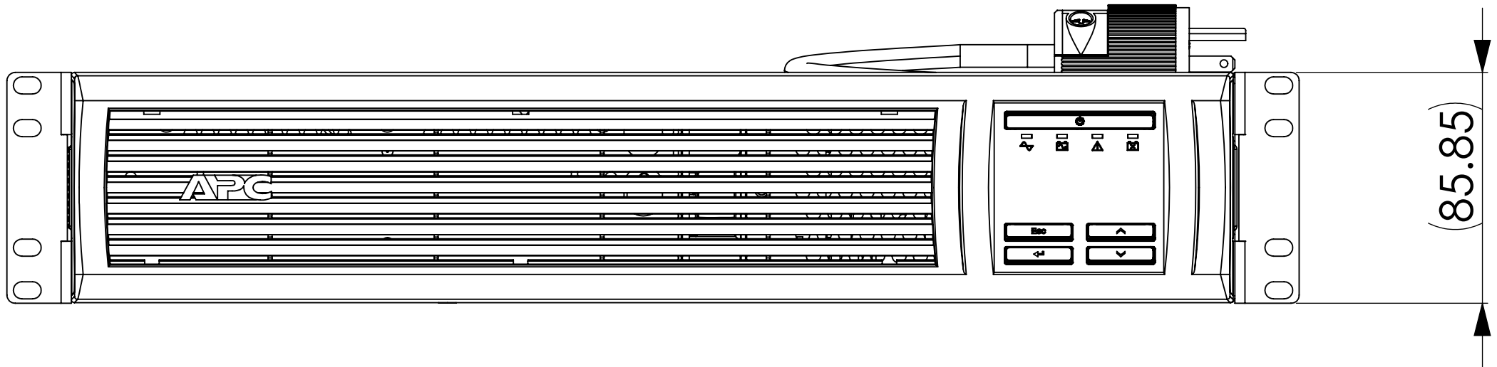
FRONT VIEW
