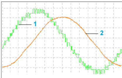
1 Voltage on motor side 2 Current on motor side
