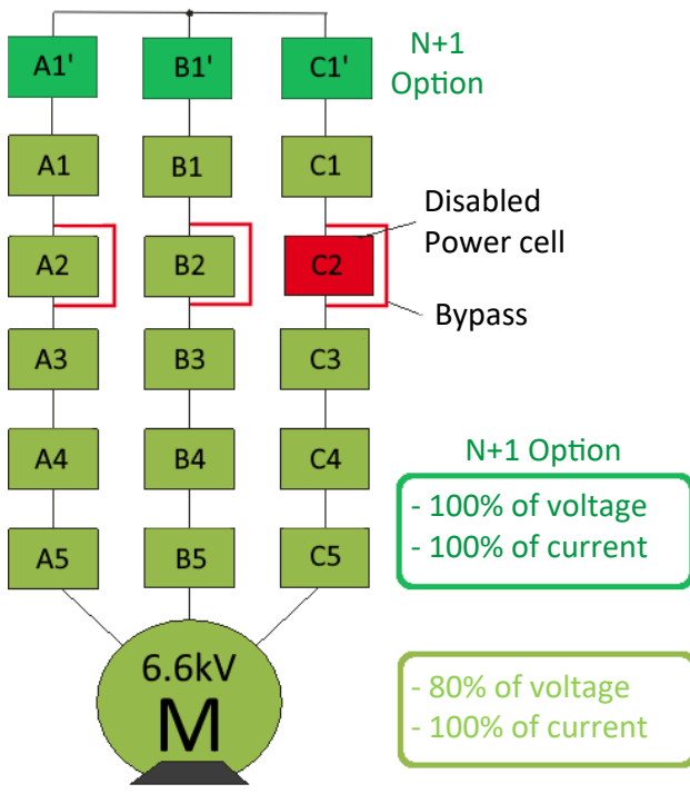
Bypass principle
