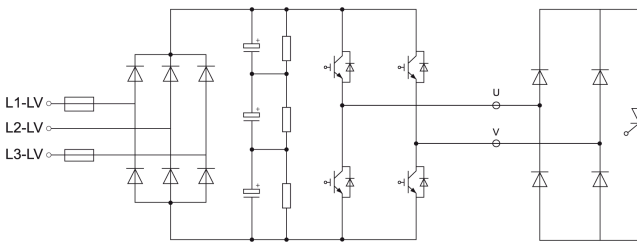
Power cell bypass circuit schematic
