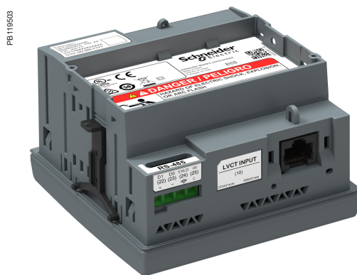
PM2220R series meter - underside view
