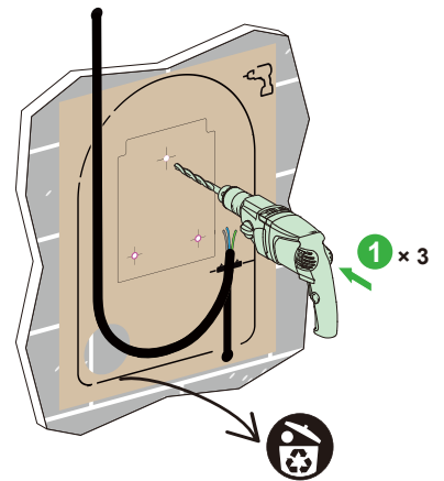
Cable entry from the top
