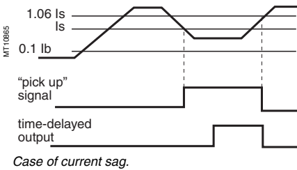
Case of current sag.
