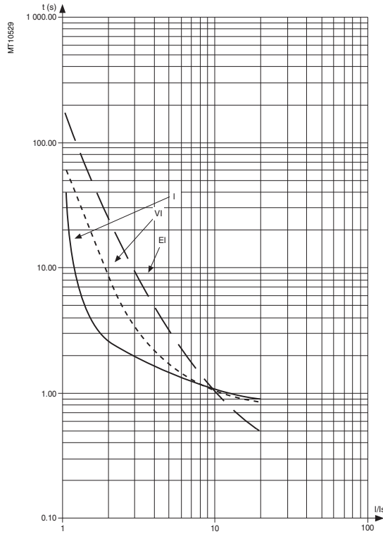
IAC curves
