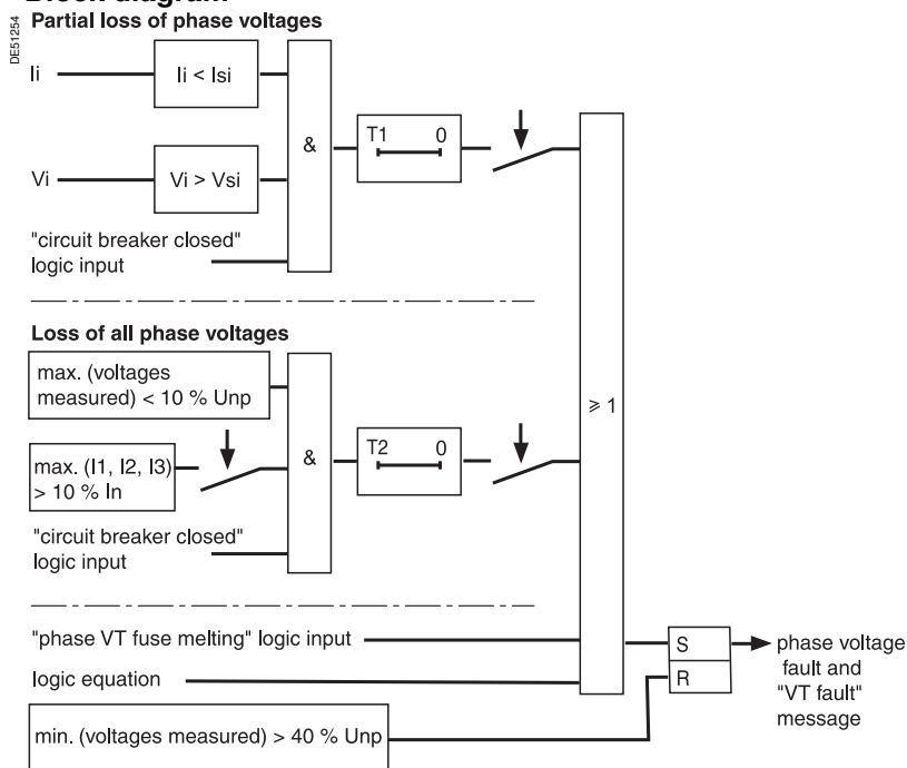
Detection of phase voltage fault.
