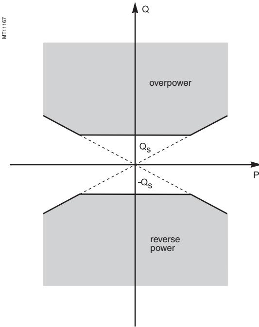
Operating zone.
