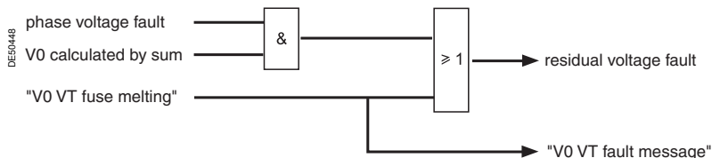
Detection of residual voltage fault.
