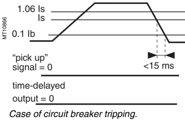
Case of circuit breaker tripping.
