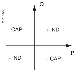
IEC convention.
