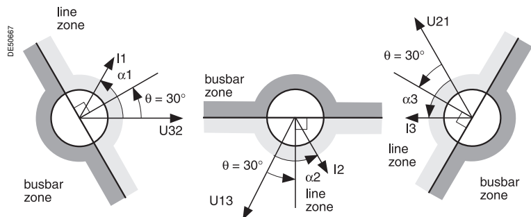
Fault tripping in line zone with \theta = 30^\circ .
