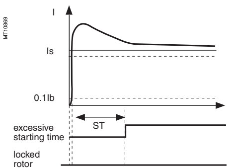
Case of excessive starting time.
