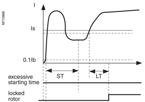
Case of locked rotor.
