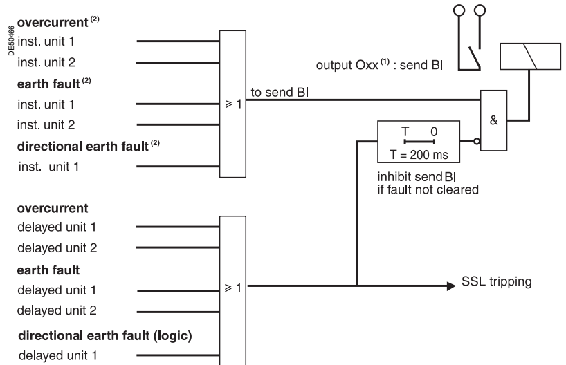
Block diagram: Sepam M40 and M41
