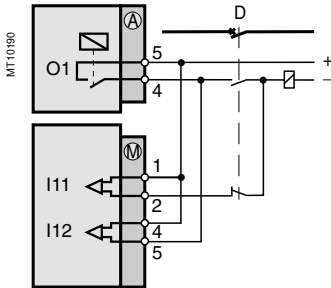
Wiring for shunt trip unit.
