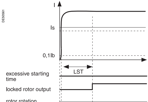
Case of starting locked rotor.
