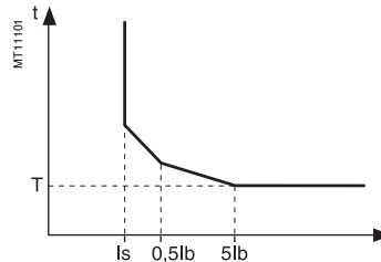
Schneider curve.
