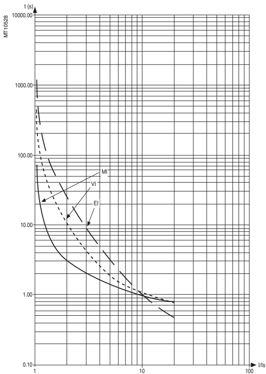
IEEE curves
