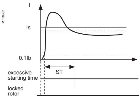
Case of normal starting.
