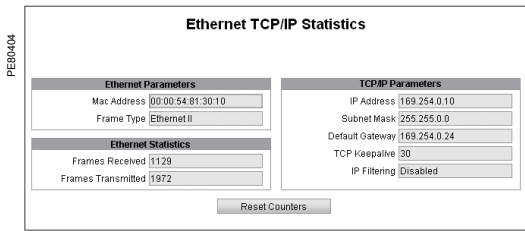
ACE850 Ethernet TCP/IP statistics.
