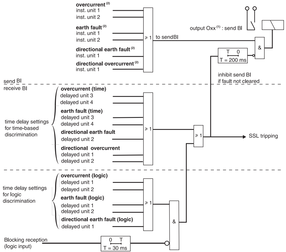
Block diagram: Sepam S40, S41, S43, S44, S50, S51, S53, S54, T40, T42, T50, T52, G40
