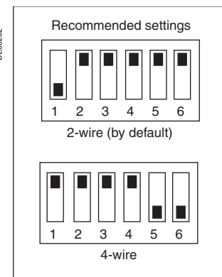
Setting the RS 485 network parameters.
