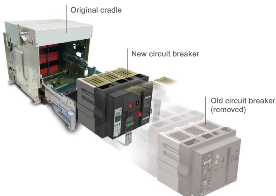
Figure: An aging circuit breaker is replaced by a modern circuit breaker, while maintaining its original cradle.
