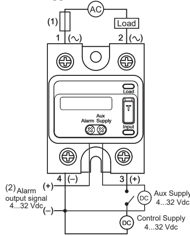
Dual Supply Connection
