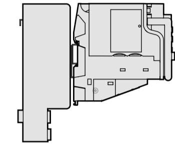
Installing the HU250 module on a PS50 enclosure
