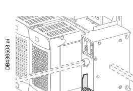
3 padlocks directly on the device
