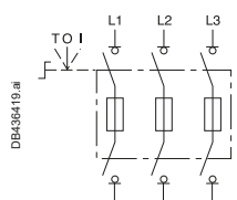
3 poles, 3 fuse-links
