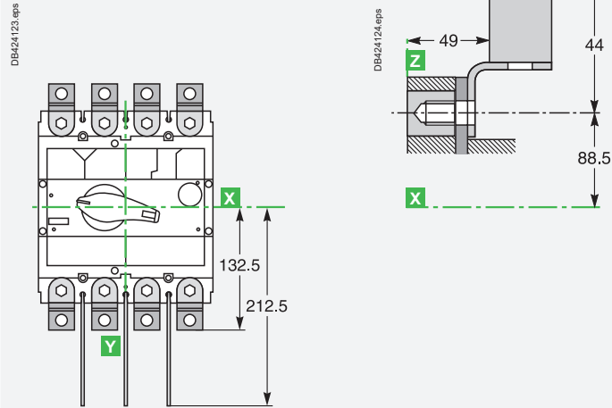
2-cable connector
