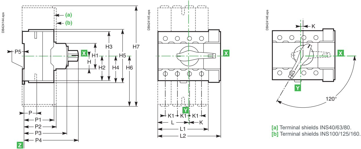
Dimensions (mm)
