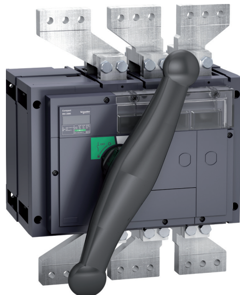
ComPact INV2500 switch-disconnector.
