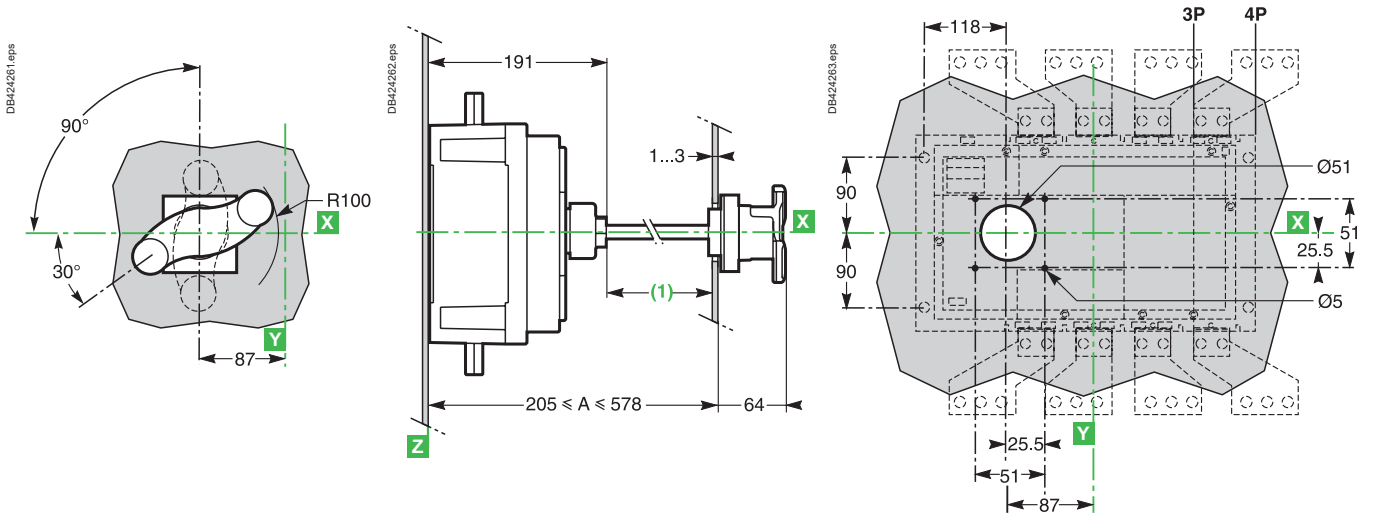
[1] Length of shaft = A - 151.
