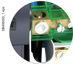
On LGY412560 and LGY416048 references. Input cabling facilitated by side terminals.
