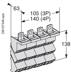
Linergy DP 250 A distribution block.
