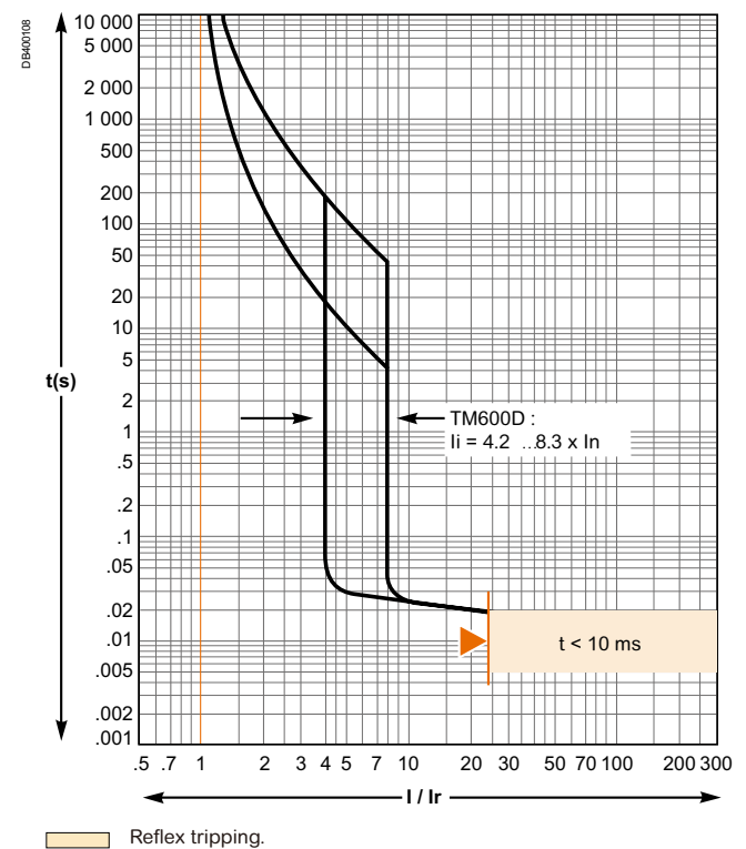
TM600D
