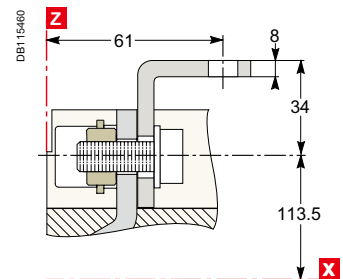
DB115460 CVS400/630
