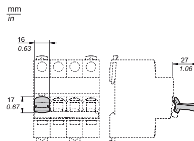
Front padlocking device
