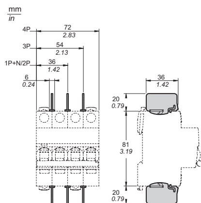
Inter-pole barrier
