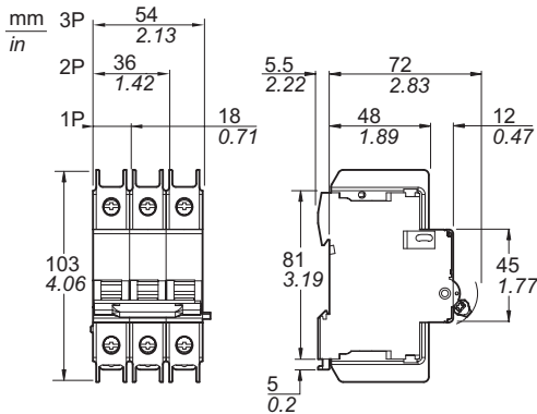
C60BP Tunnel terminal
