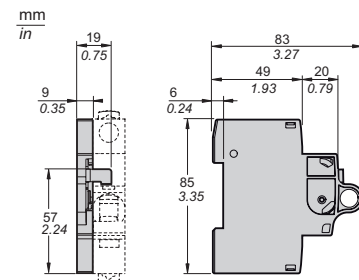
Side padlocking device
