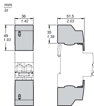
Terminal shield 2P
