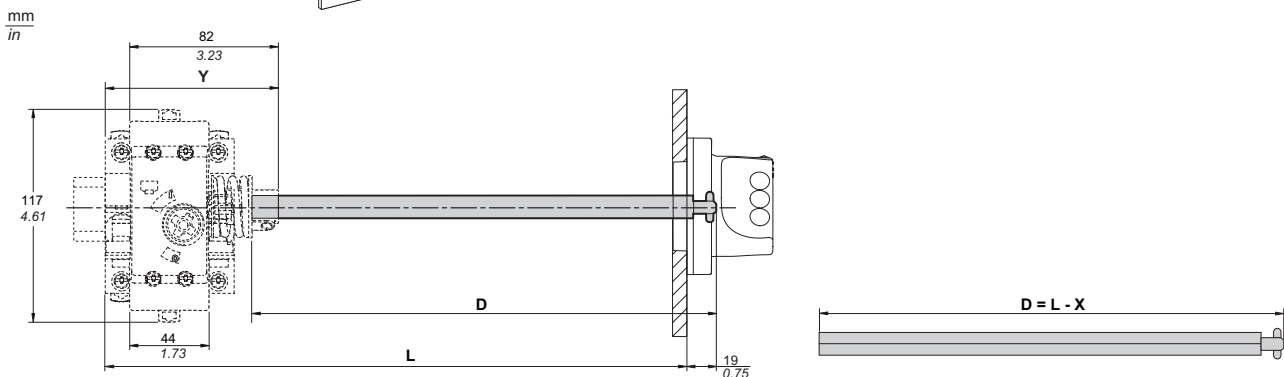
Rotary handle: side mounted control
