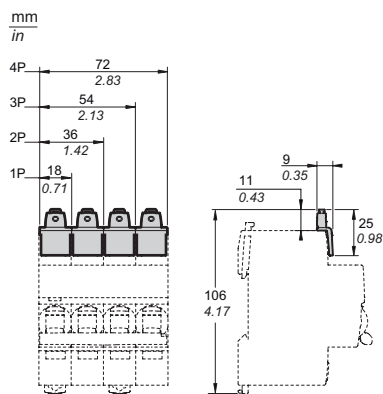
Screw shield 4P (A9A26981)
