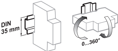
Clip on DIN rail 35 mm. Indifferent position of installation.
