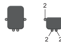
2 Screw: M3x8 ISO 14583, torque 0.6 Nm (5.31 lbf-in)
