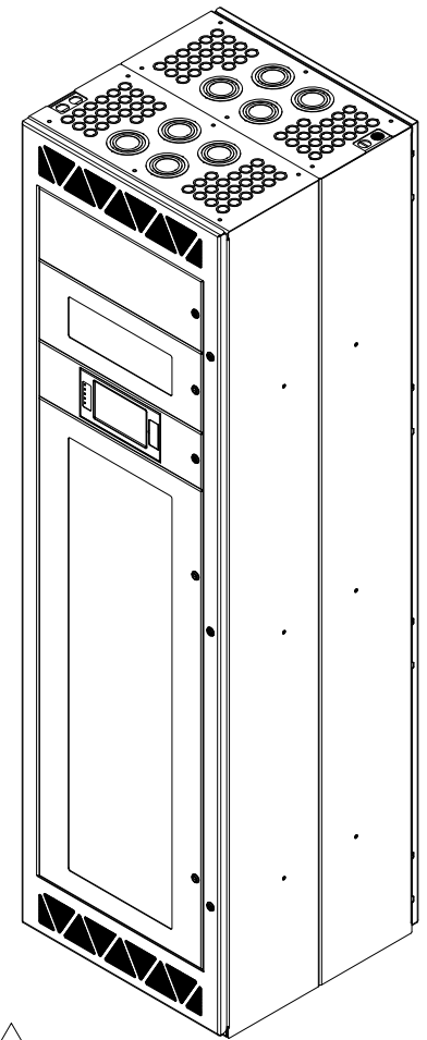
ISOMETRIC VIEW – BACK TO BACK ANCHORING
