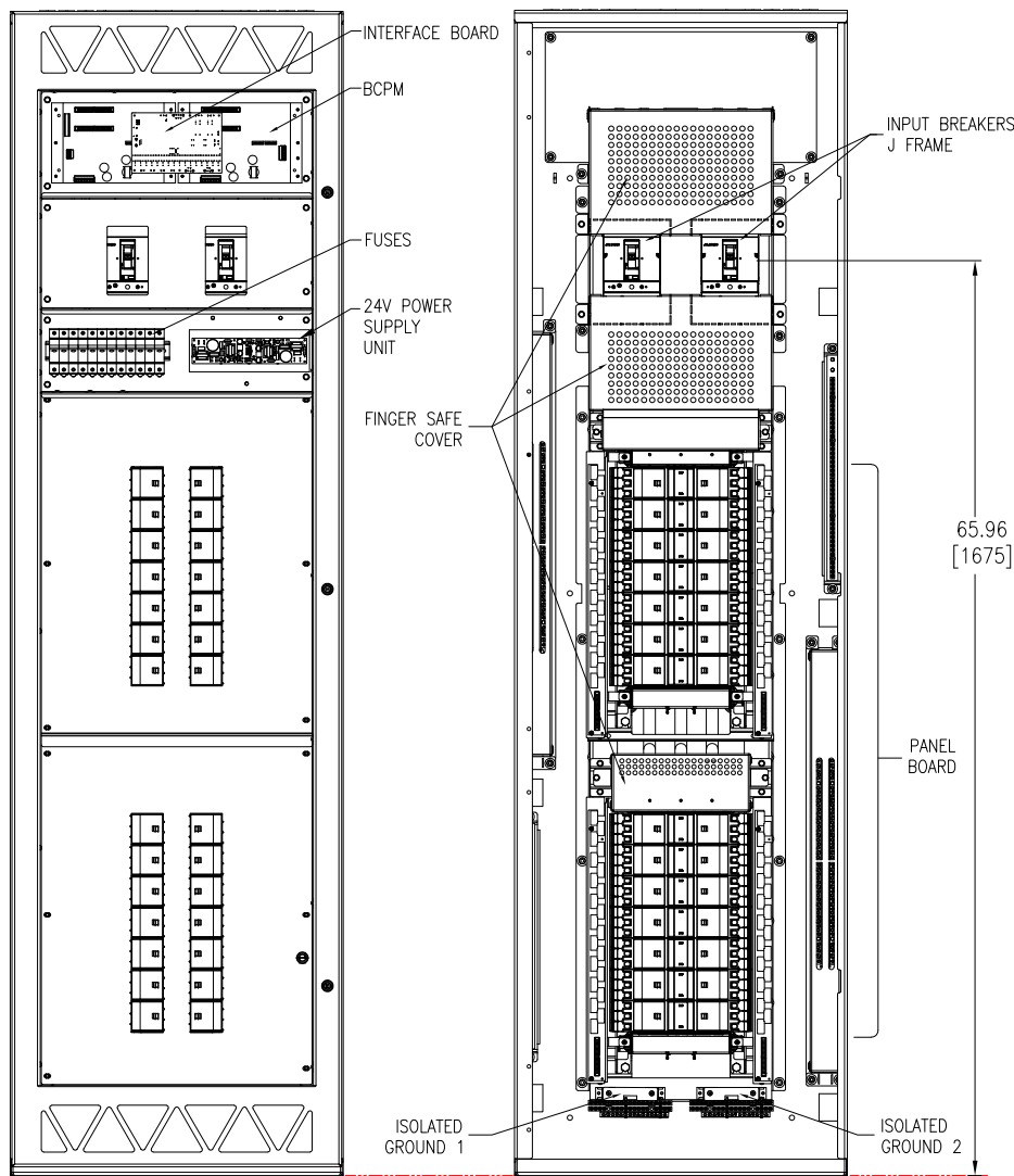
INTERNAL FRONT VIEW-IP2X 42 (DEAD FRONT DOOR COVERS REMOVED)
