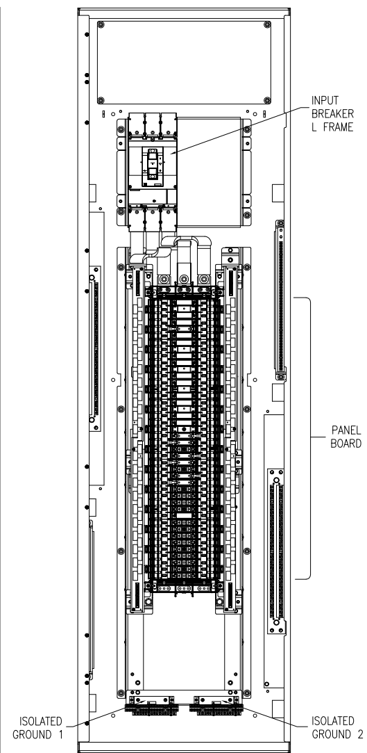
INTERNAL FRONT VIEW-NQ 84 (DEAD FRONT DOOR REMOVED)
