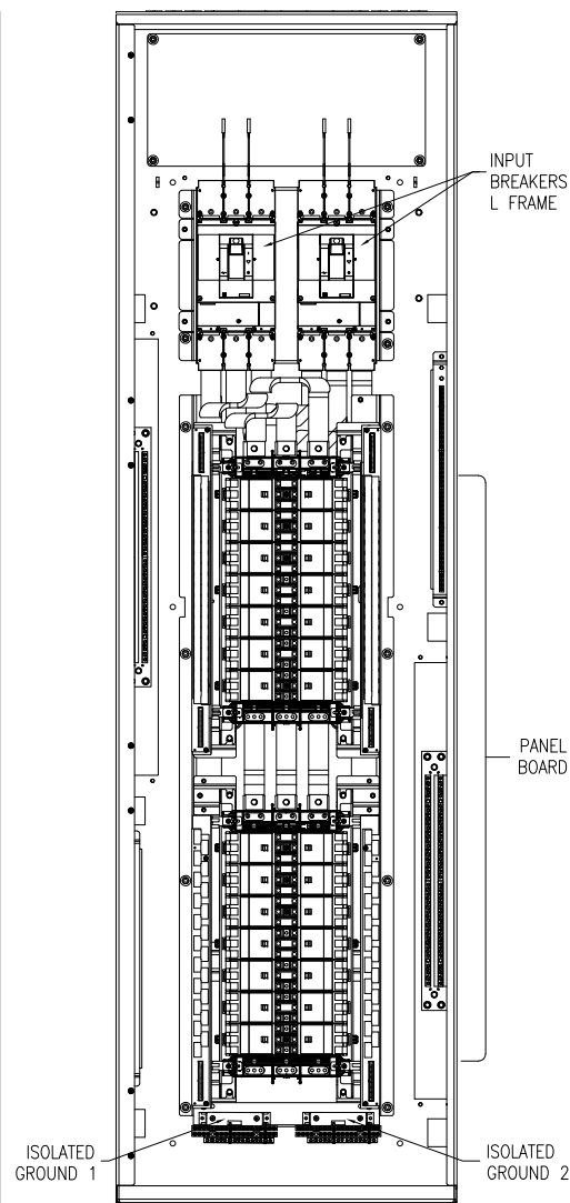
INTERNAL FRONT VIEW-NQ 42 (DEAD FRONT DOOR REMOVED)
