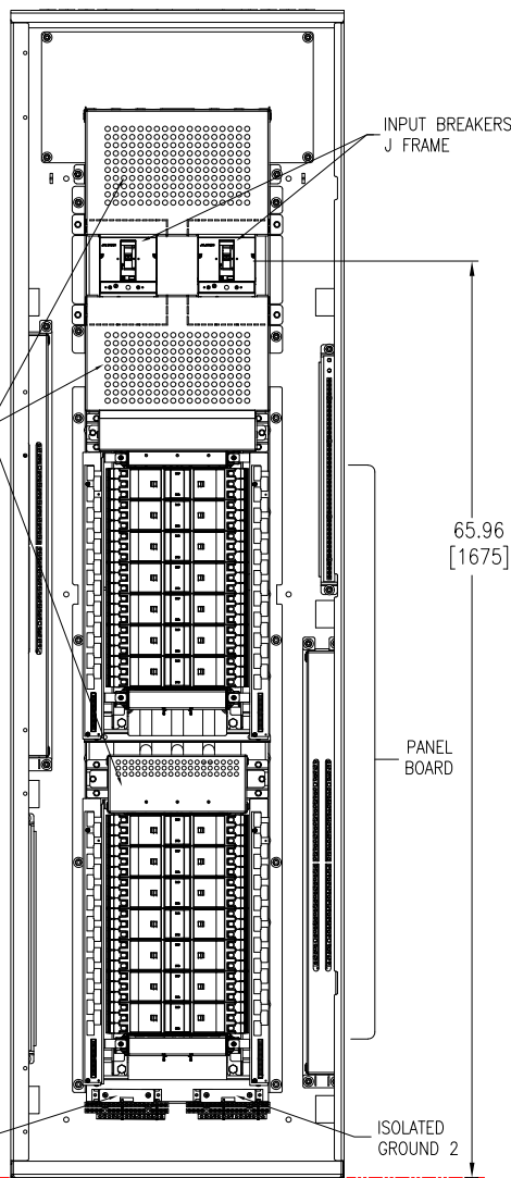
INTERNAL FRONT VIEW-IP2X 42 (DEAD FRONT DOOR REMOVED)
