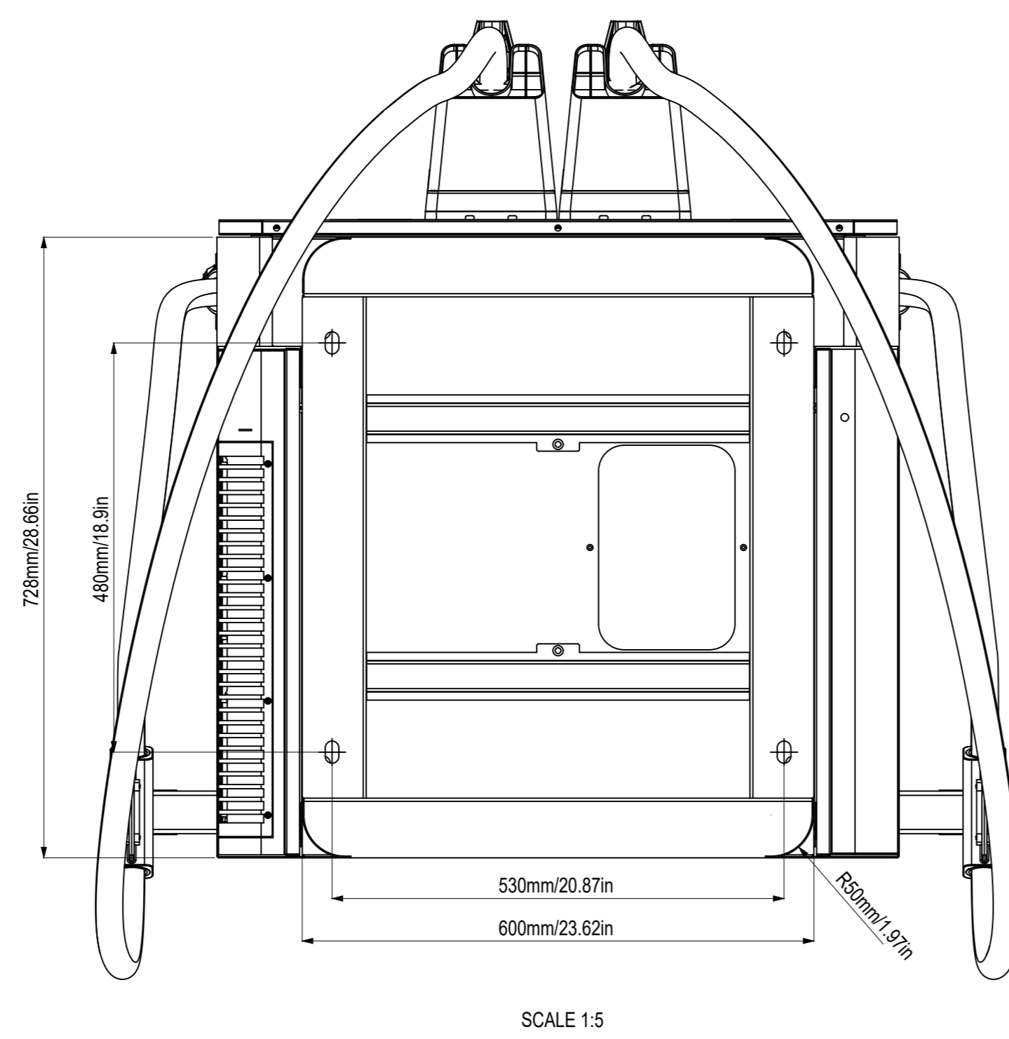
SCALE 1:5
