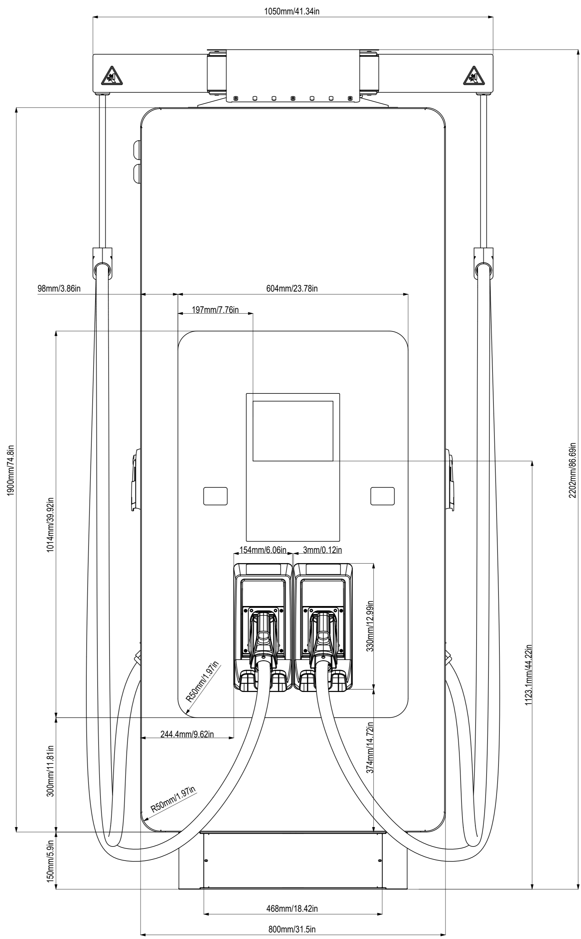
SCALE 1:5
