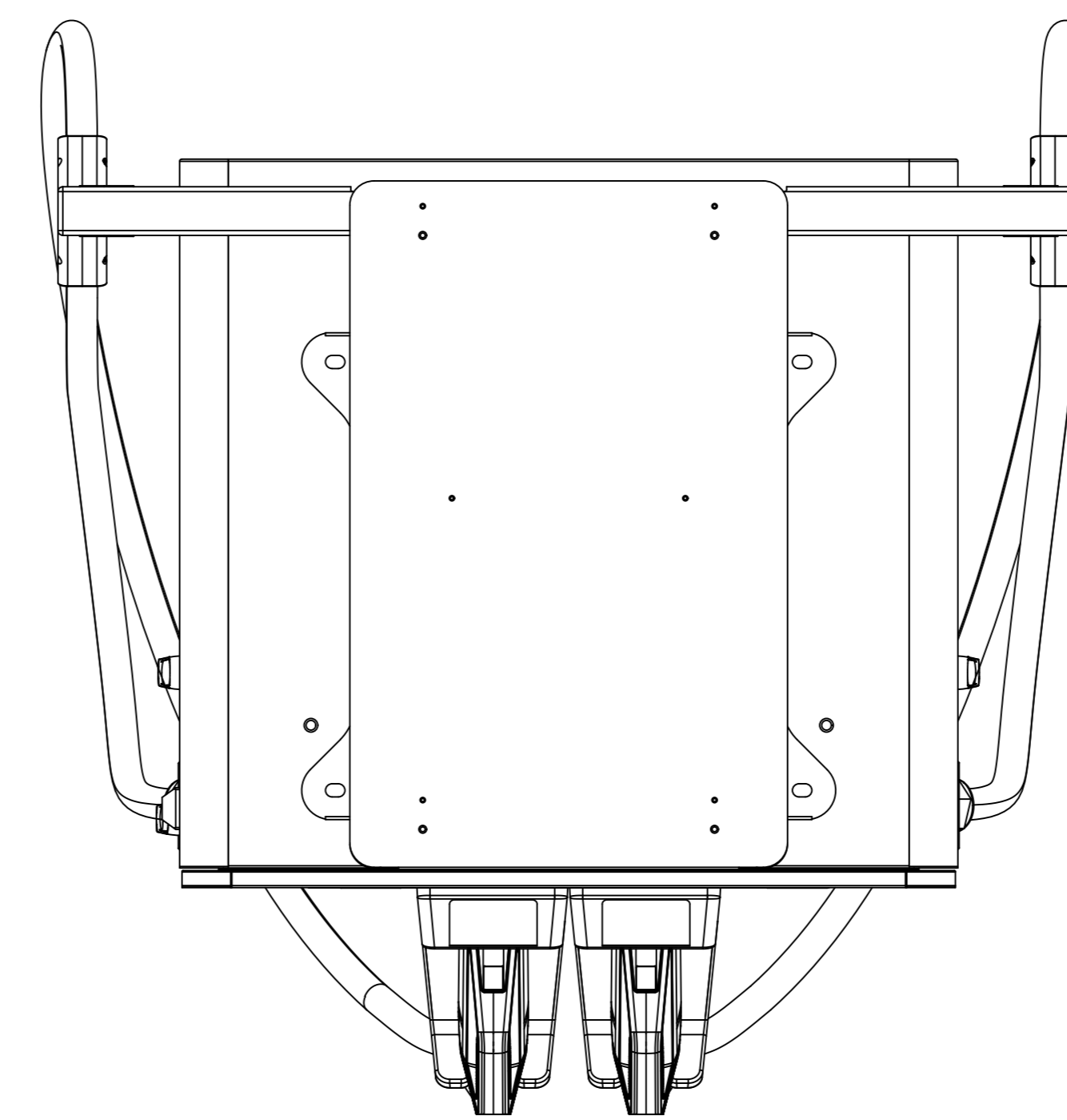
SCALE 1:5
