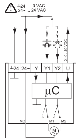
Wiring for 3-point control
