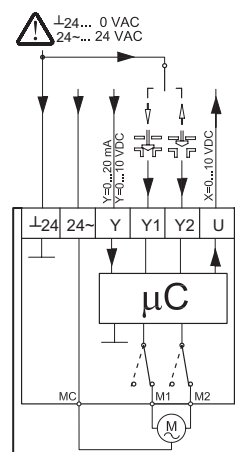
Wiring for modulating control
