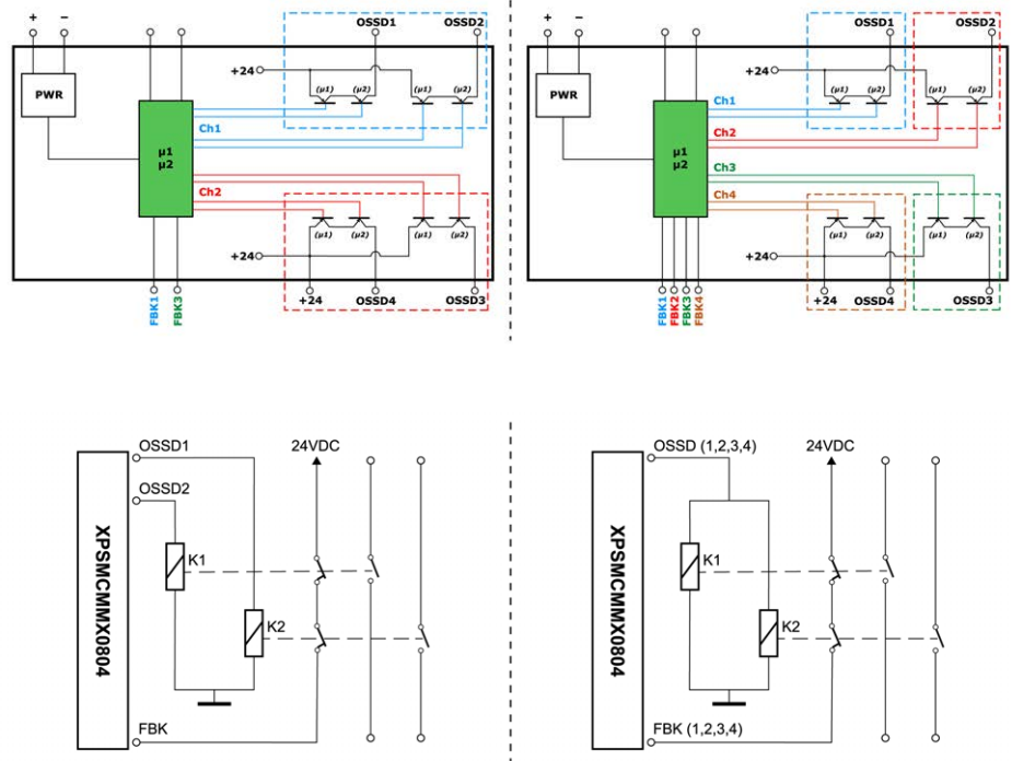
Dual channel OSSD configuration with 2 dual channel outputs, safety category SIL3/PL e: EN 61508:2010
