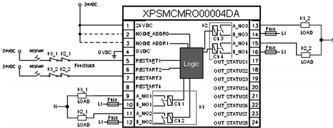
Category 4 wiring
