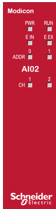
XPSMCMIAI0200(G)
