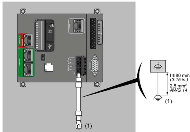
(1) Functional earth ground (FE)
