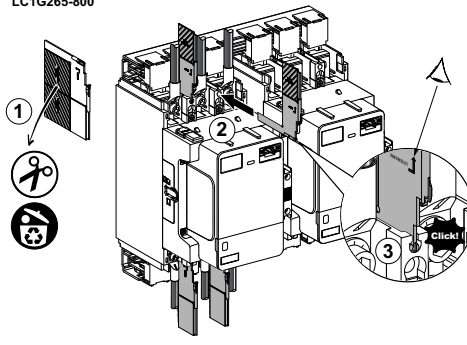
LC1G265-800
