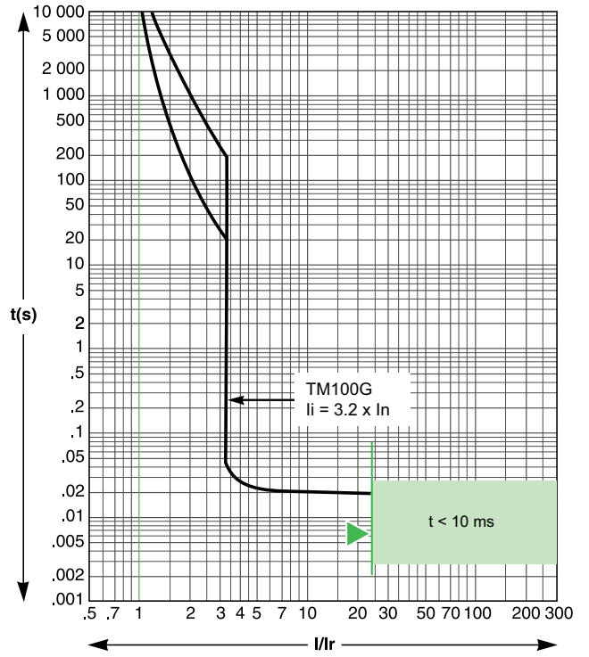
TM100G
