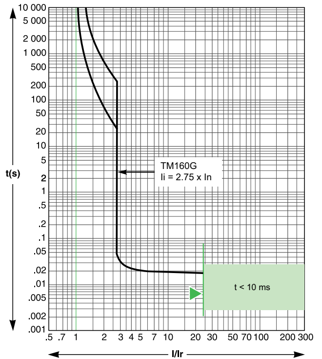
TM160G
