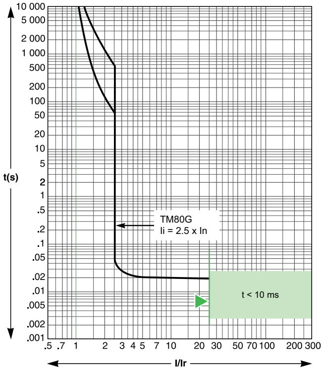
TM80G
