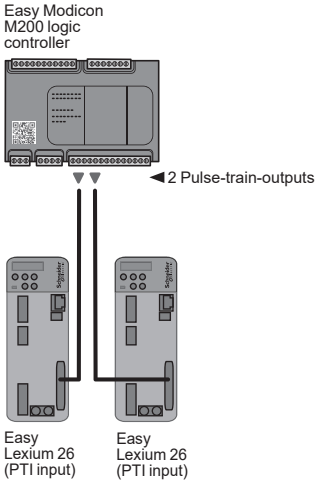
Example of architecture with control by Easy Modicon M200 logic controller
