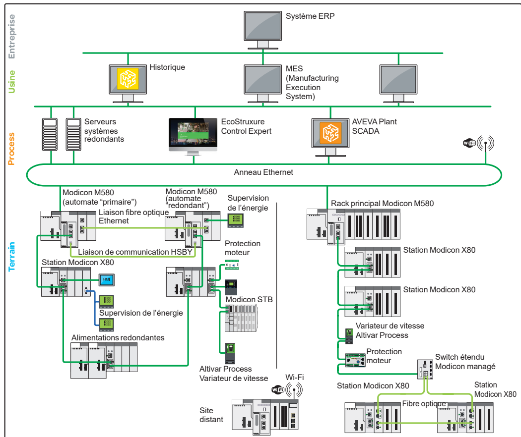
Architecture type (3)
