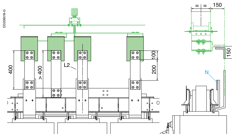
KTC●●●●EL●5 with angle bracket KTB0000YE
