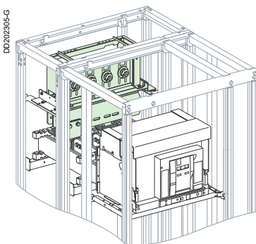
Rear connection
