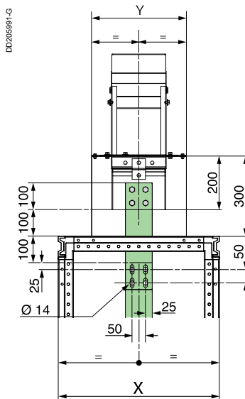
Vertical incomer
