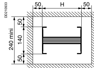
Flat passage through partition wall
