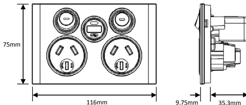
Dimensions of 4025USBC DGPO with USB Charger
