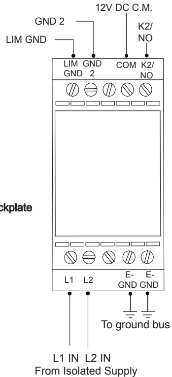
Test Simulator Module for LIM
