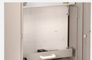
Hinged and moulded panel with provision for two meters inside
