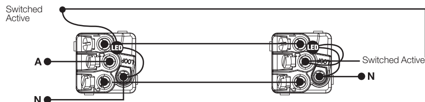
Two-way switching, Neutral present at the switch LED 'ON' switch 'ON'
