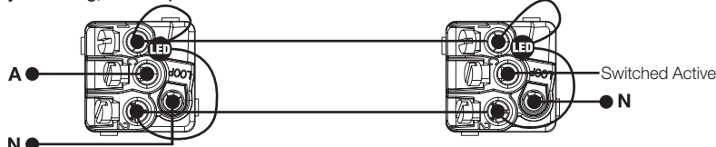
Two-way switching, Neutral present at the switch LED 'ON' switch 'OFF'
