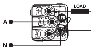
Wire the LED as a POWER AVAILABILITY INDICATOR LED ON, switch OFF (using Neutral)
