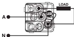
Wire the LED as a SWITCH LOCATOR LED permanently ON
