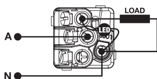
LED 'ON' switch 'ON' (using Neutral)
