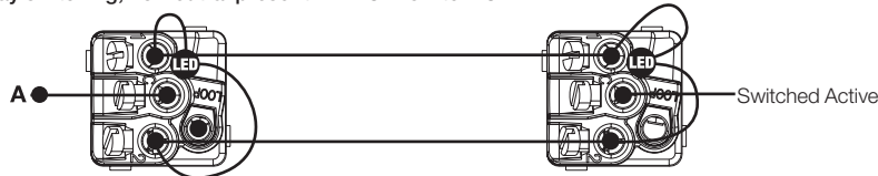
Two-way switching, no Neutral present LED 'ON' switch 'OFF'
