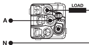
LED ON, switch OFF, (no Neutral required)
