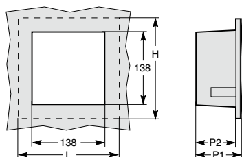
Varlogic NR6/NR12 : 150 x 150 x 70/60 mm
