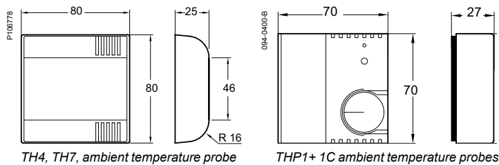
TH4, TH7, ambient temperature probe
