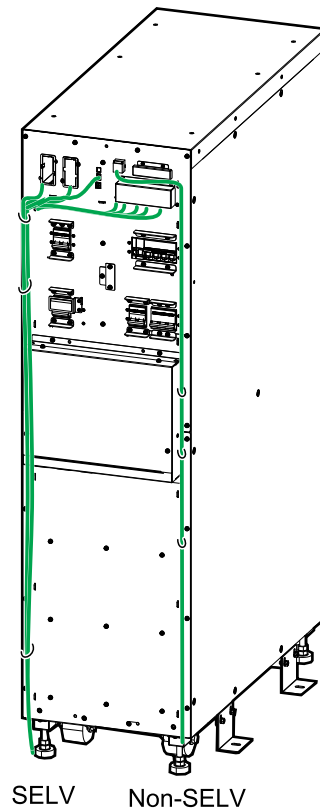
SELV and Non-SELV Cable Routing for 10 - 20 kVA 3:1 UPS
