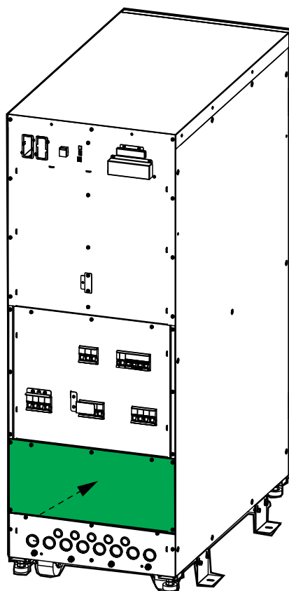
Rear View of 30 kVA 3:1 UPS
