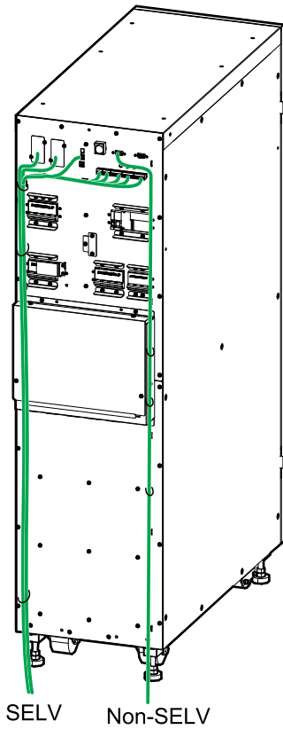
SELV and Non-SELV Cable Routing for 10 - 20 kVA 3:3 UPS
