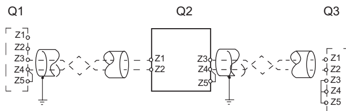
Figure 14 – ZSI Wiring
