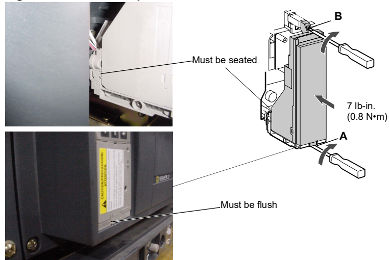
Figure 21 – Install Trip Unit
