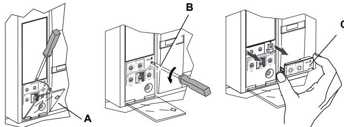
Figure 23 – Remove Adjustable Rating Plug
