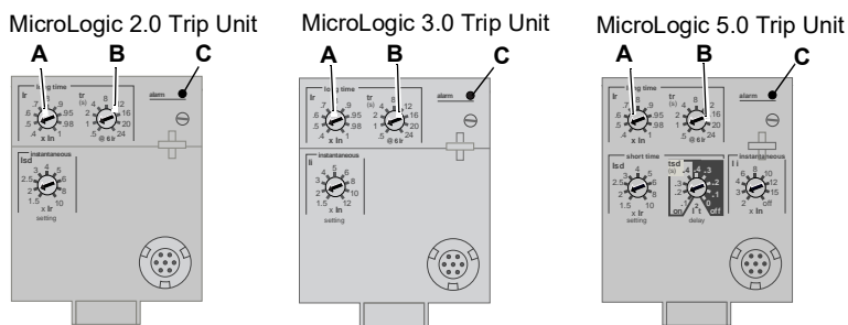
Figure 5 – Long-Time Protection Switches
