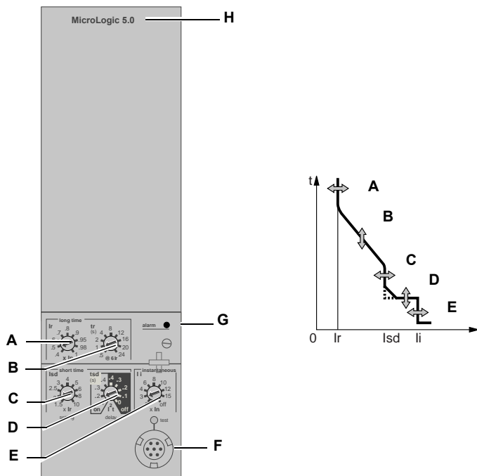
Figure 4 – MicroLogic 5.0 Trip Unit
