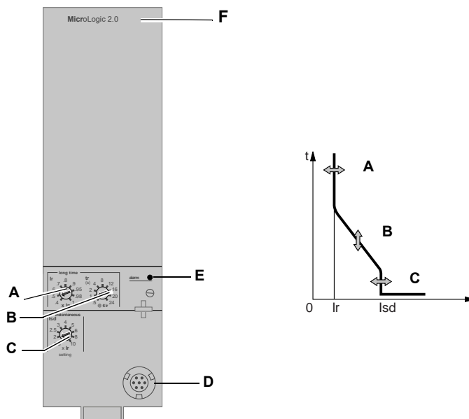
Figure 2 – MicroLogic 2.0 Trip Unit
