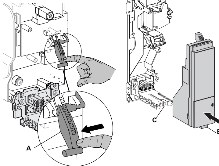
Figure 20 – Install Trip Unit
