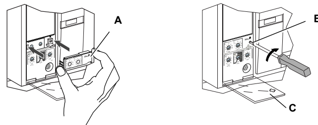
Figure 24 – Install New Adjustable Rating Plug
