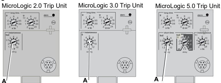
Figure 7 – Instantaneous Protection Switches
