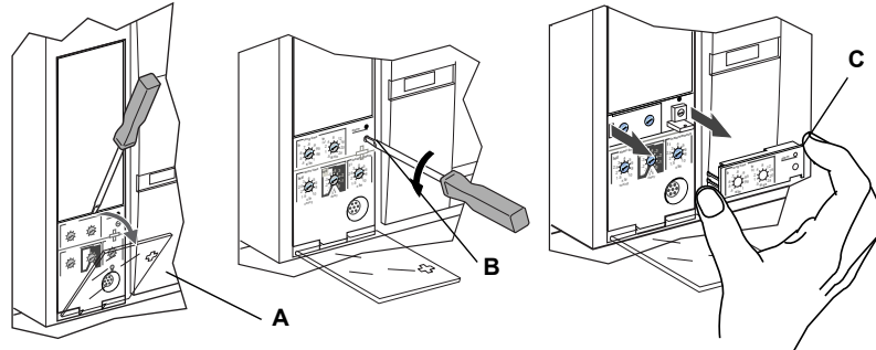
Figure 18 – Remove Adjustable Rating Plug
