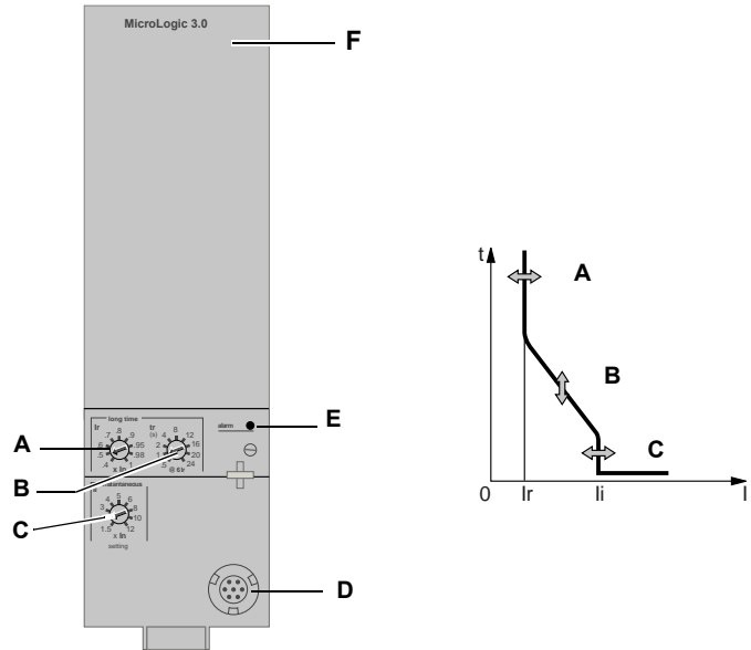
Figure 3 – MicroLogic 3.0 Trip Unit
