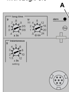
Figure 8 – Voyant de surcharge
