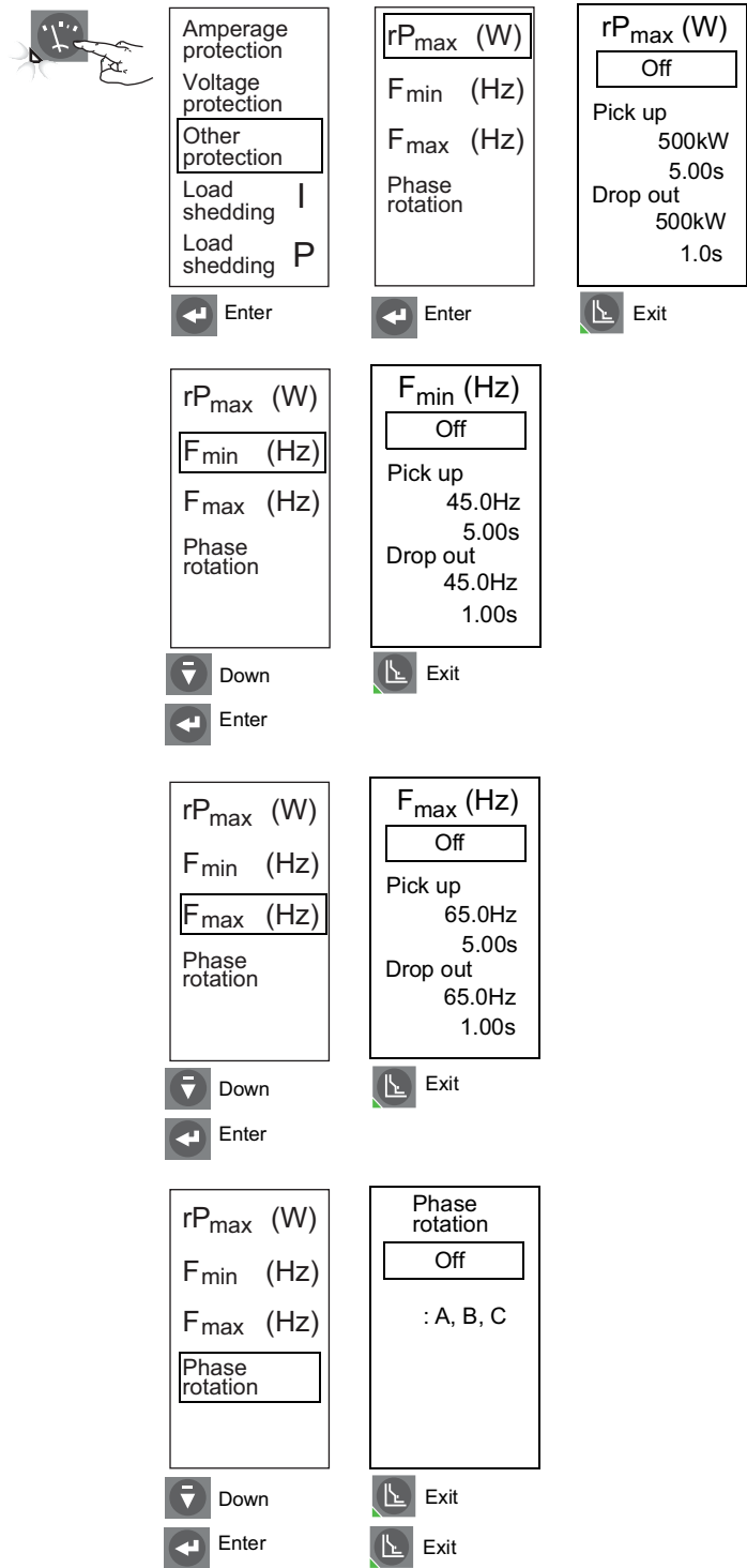
Figure 87 - Check Other Protection
