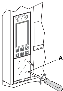
Figure 69 - Test Equipment Ground-Fault Trip Function
