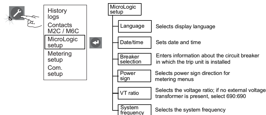
Figure 8 - MicroLogic Setup
