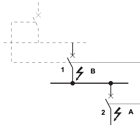
Figure 16 - Zone-selective Interlocking
