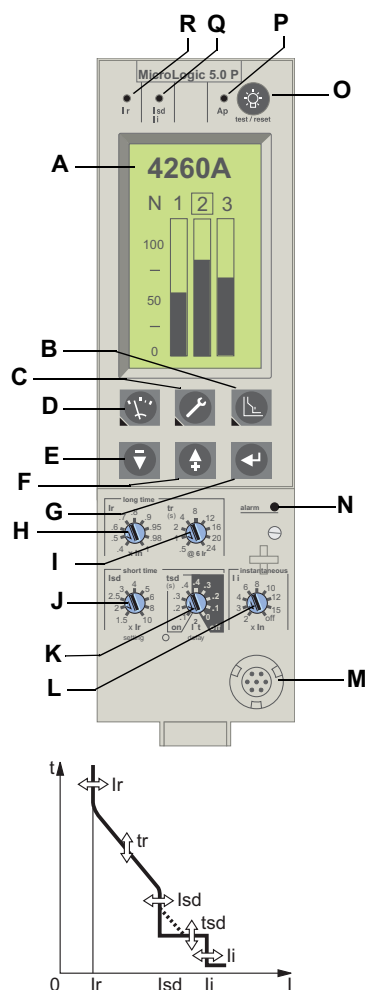
Figure 2 - 5.0P Trip Unit
