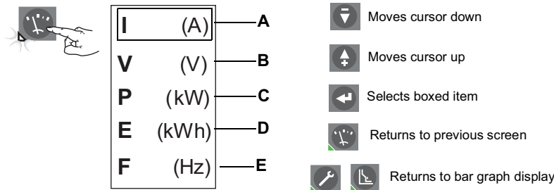
Figure 34 - Metering Menu
