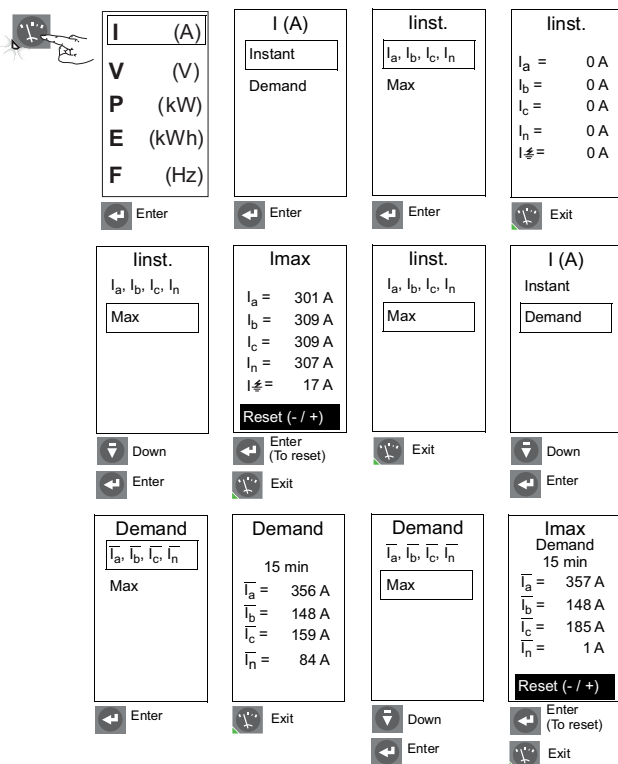
Figure 72 - Check Current Levels
