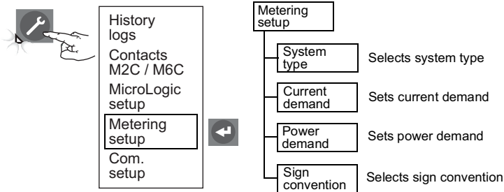
Figure 33 - Metering Setup
