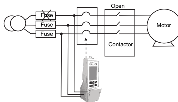
Figure 105 - Circuit Configuration 1
