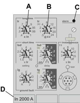
MicroLogic 6.0P Trip Unit
