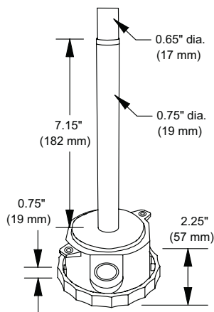
EHD110 Series
