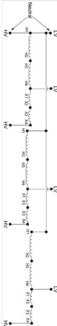
Wiring Diagram 10
