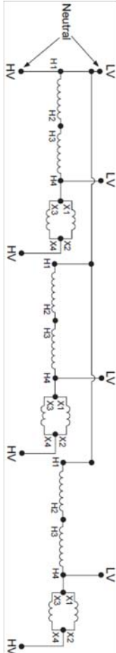
Wiring Diagram 9
