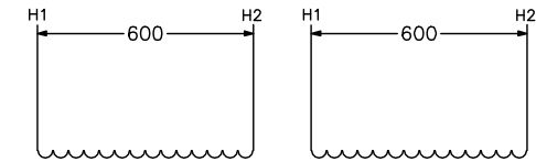
SERIES CONNECTION PARALLEL CONNECTION 240 X 480 VOLT PRIMARY
