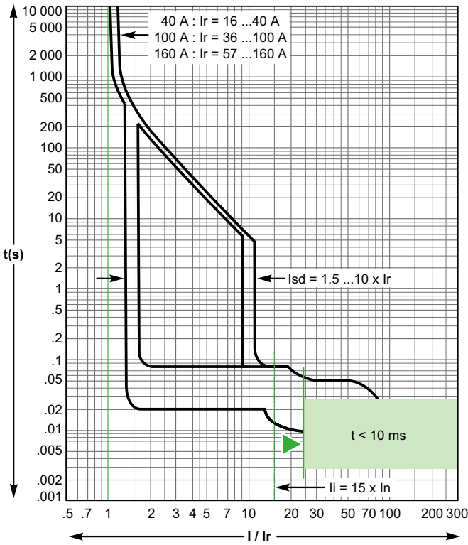
Micrologic 2.2 - 40... 160 A
