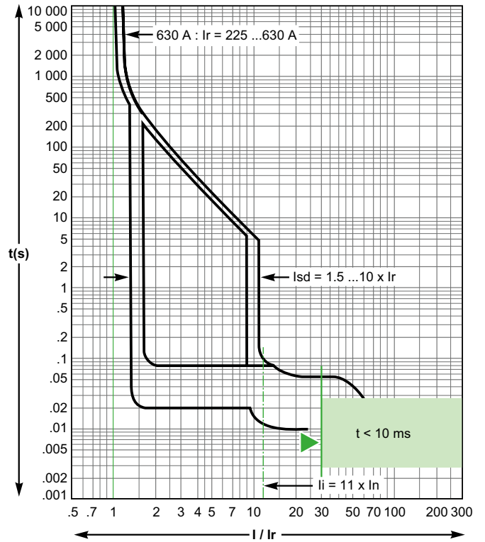
Micrologic 2.3 - 630 A
