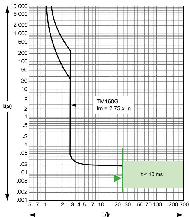
TM160G
