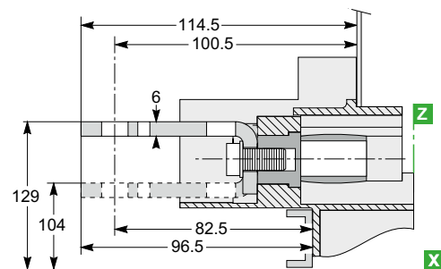
NSX400/630
