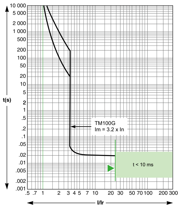
TM100G
