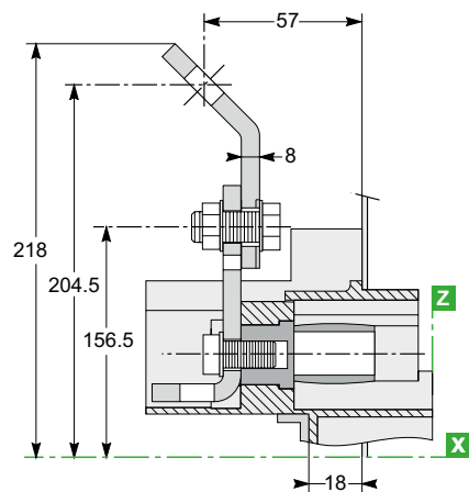
NSX400/630
