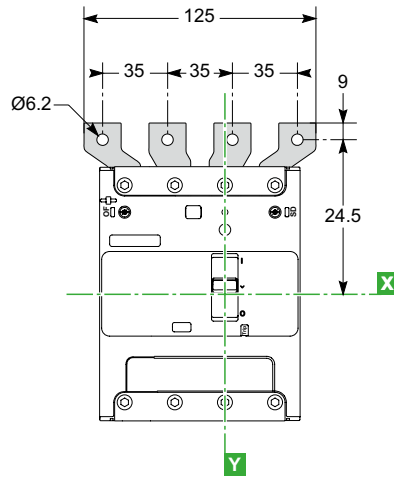
4P
