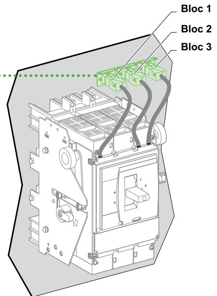
ComPact NSX400/630.
