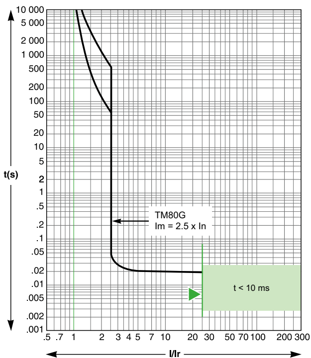
TM80G
