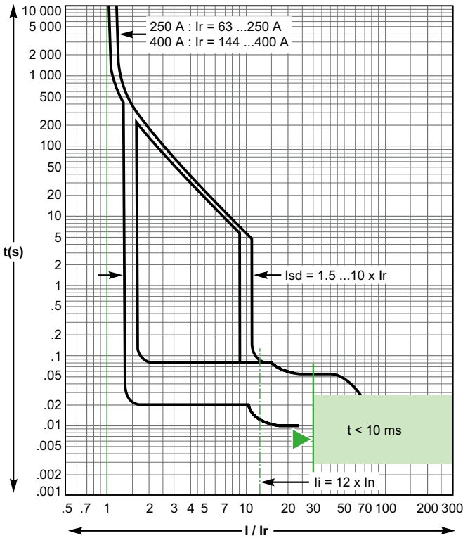
Micrologic 2.3 - 250 ... 400 A
