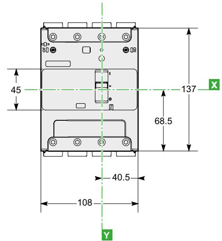
4P
