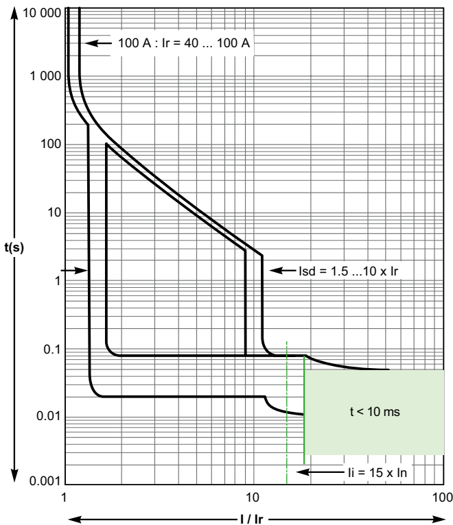
100 A
