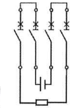
250/320/400/500/600 4P 串法1 (750Vdc)
