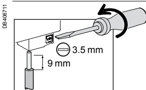
Connection by tunnel terminal with guard
