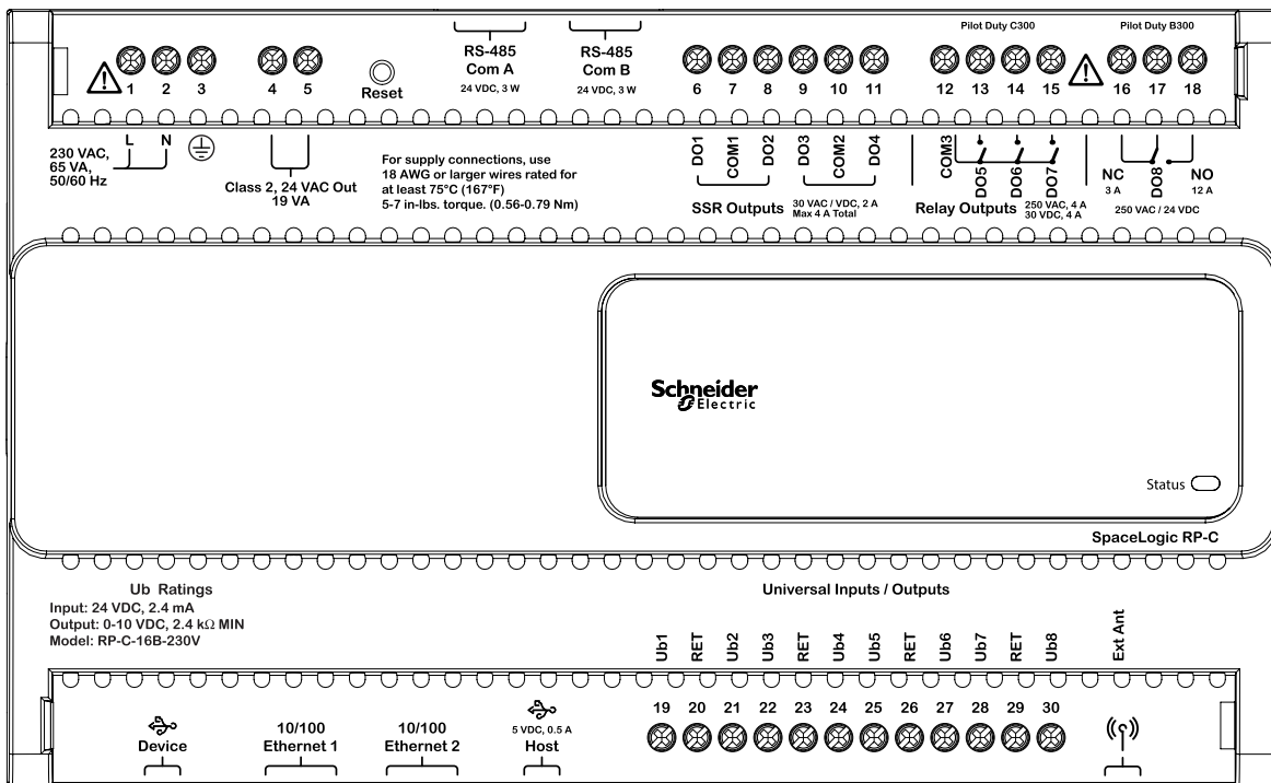
RP-C-16B-F-230V model (230 VAC)
