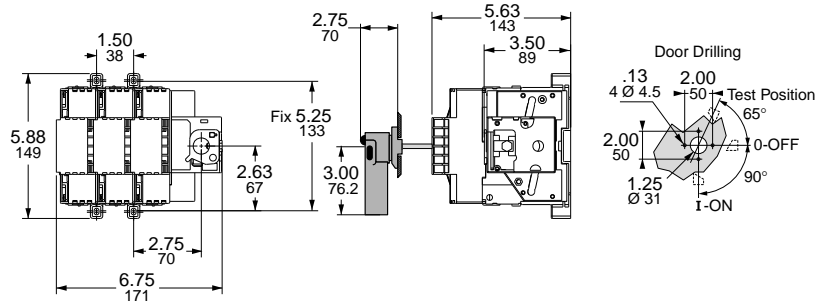
GS1EU3/GS1GU3, 30 and 60 A (Class J)
