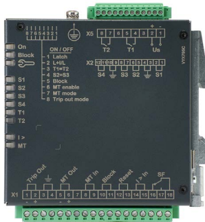
V125 Arc Flash Protection Unit
