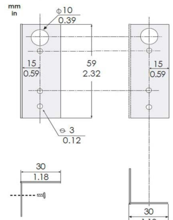
VYX 002 Surface Mounting Plate for sensors
