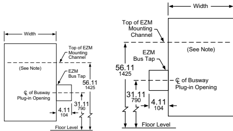
EZM 3 Phase Busway Side Tap Right EZM 3 Phase Busway Side Tap Left
