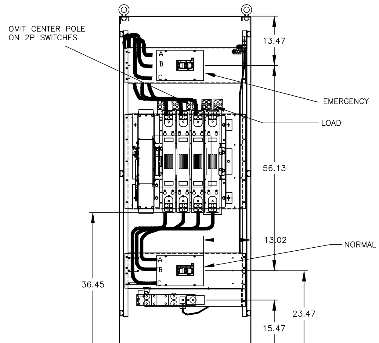
FRONT ELEVATION
