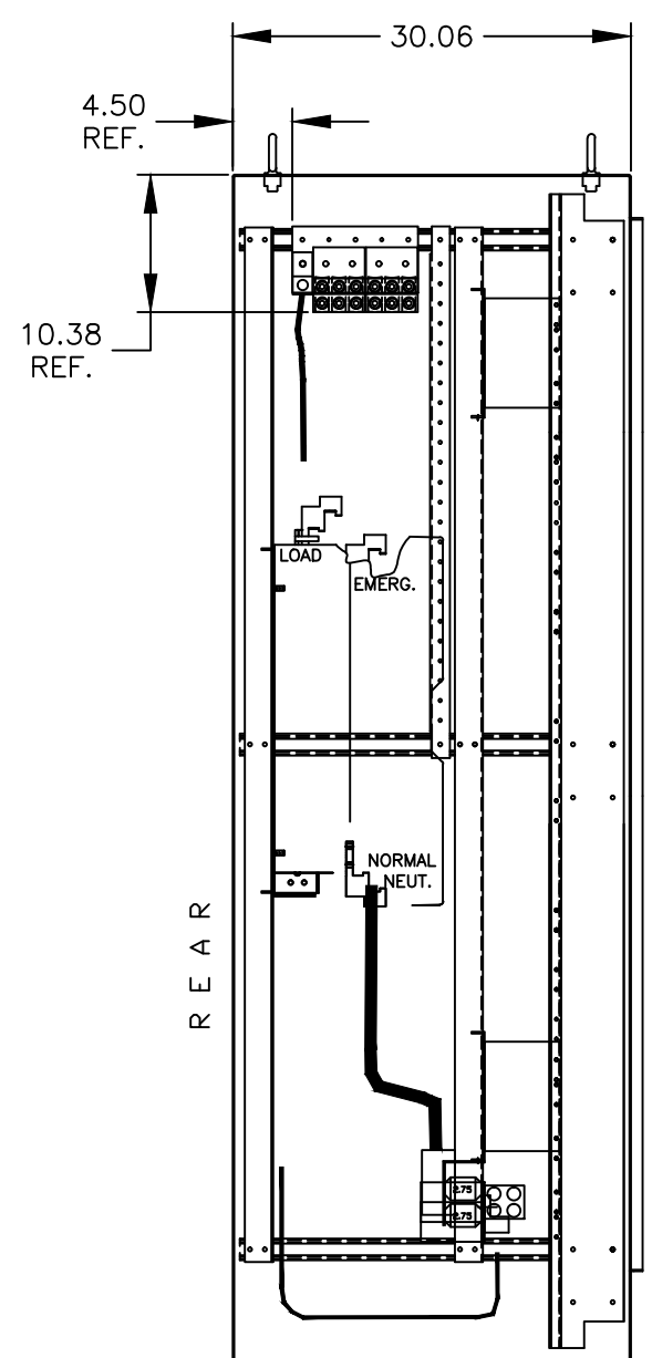
SIDE SECTION VIEW
