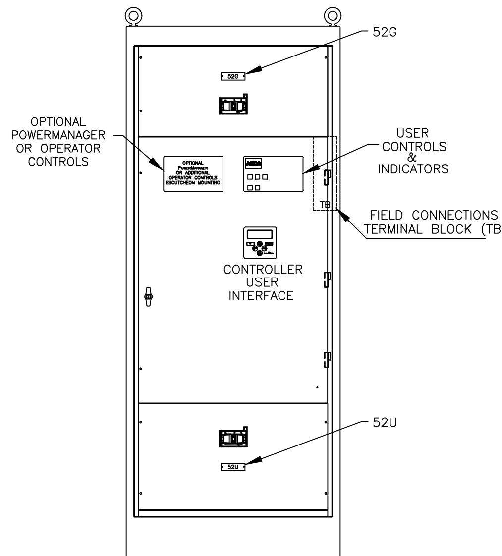
FRONT VIEW WITHOUT DOOR 7000 SERIES
