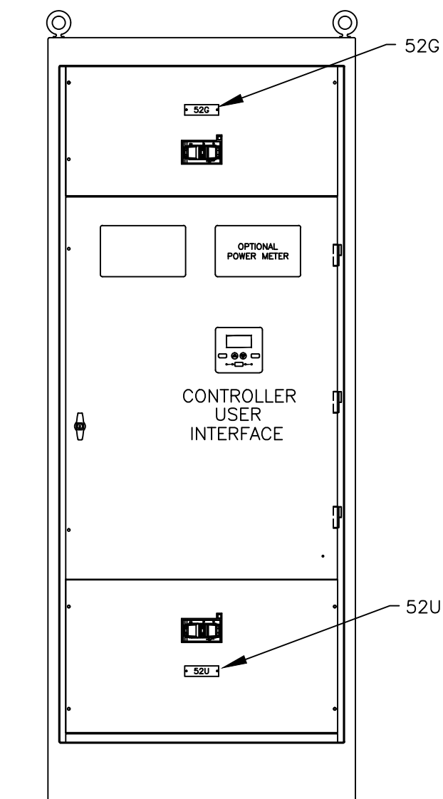
FRONT VIEW WITHOUT DOOR 300 SERIES
