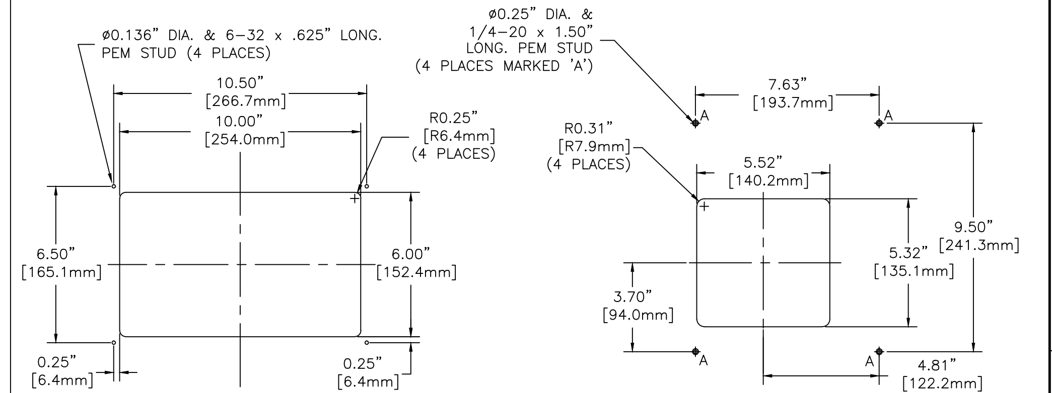
DETAIL A -1 (FOR TYPE 1)
