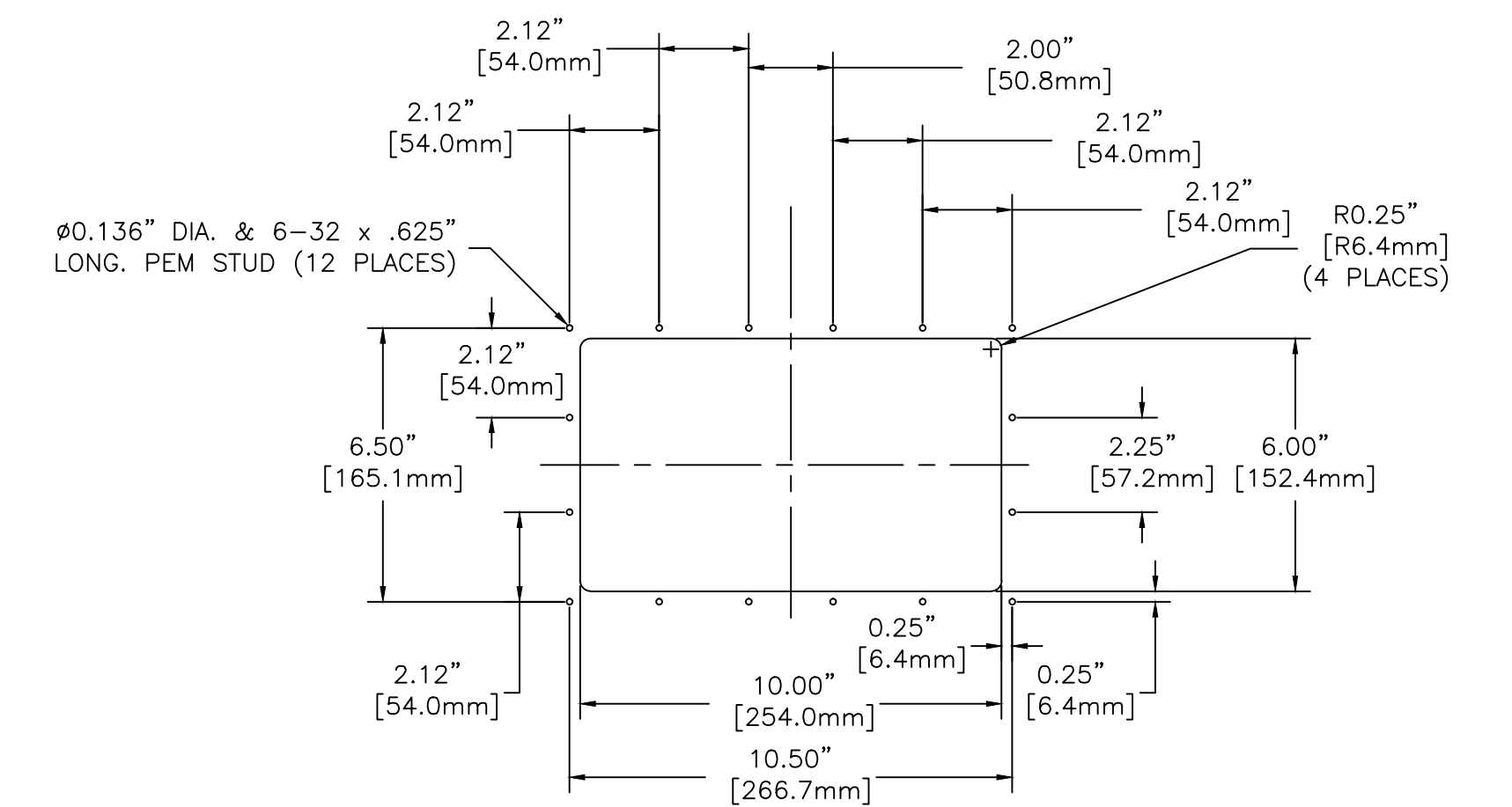
DETAIL A -2 (FOR TYPE 3R, 12 & 4)
