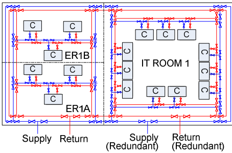
Piping inside electrical and IT rooms (1 of 4)
