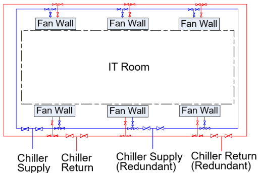
IT Room 1A Piping
