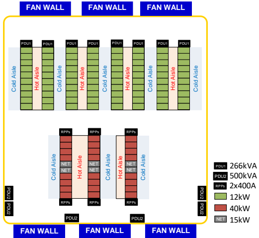
IT Room 1A Layout
