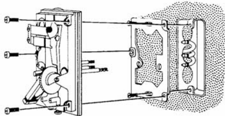
Figure-2 Mounting Thermostat to Electrical Box.
