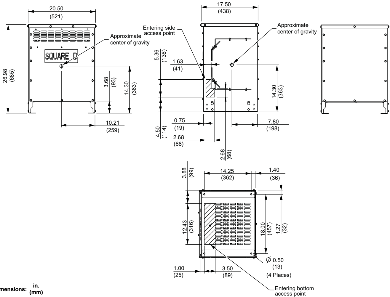
Figure 7: Enclosure 17K
