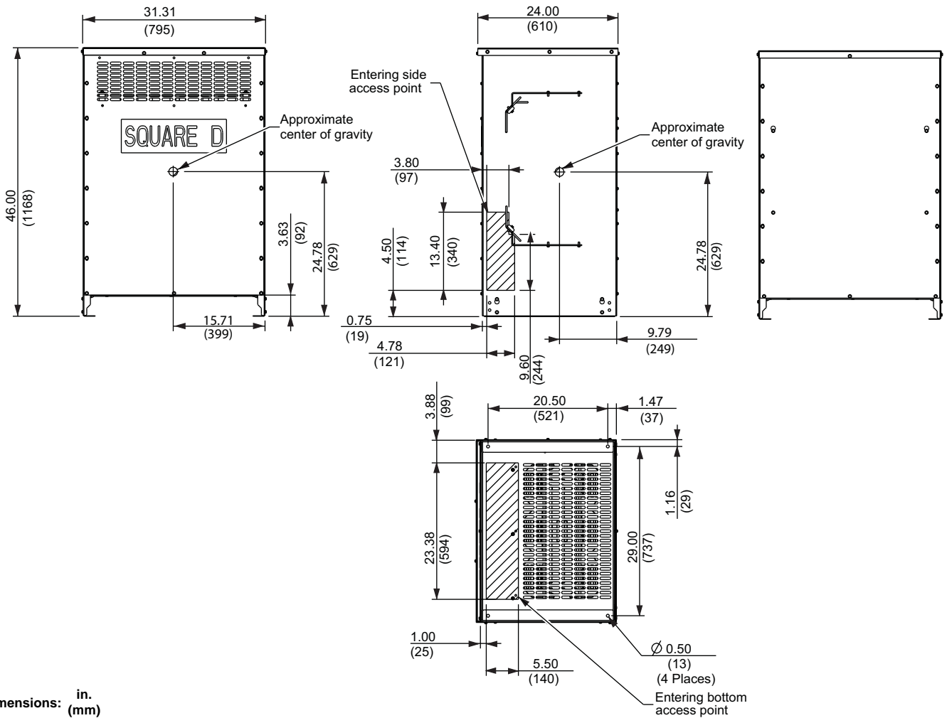
Figure 10: Enclosure 21K
