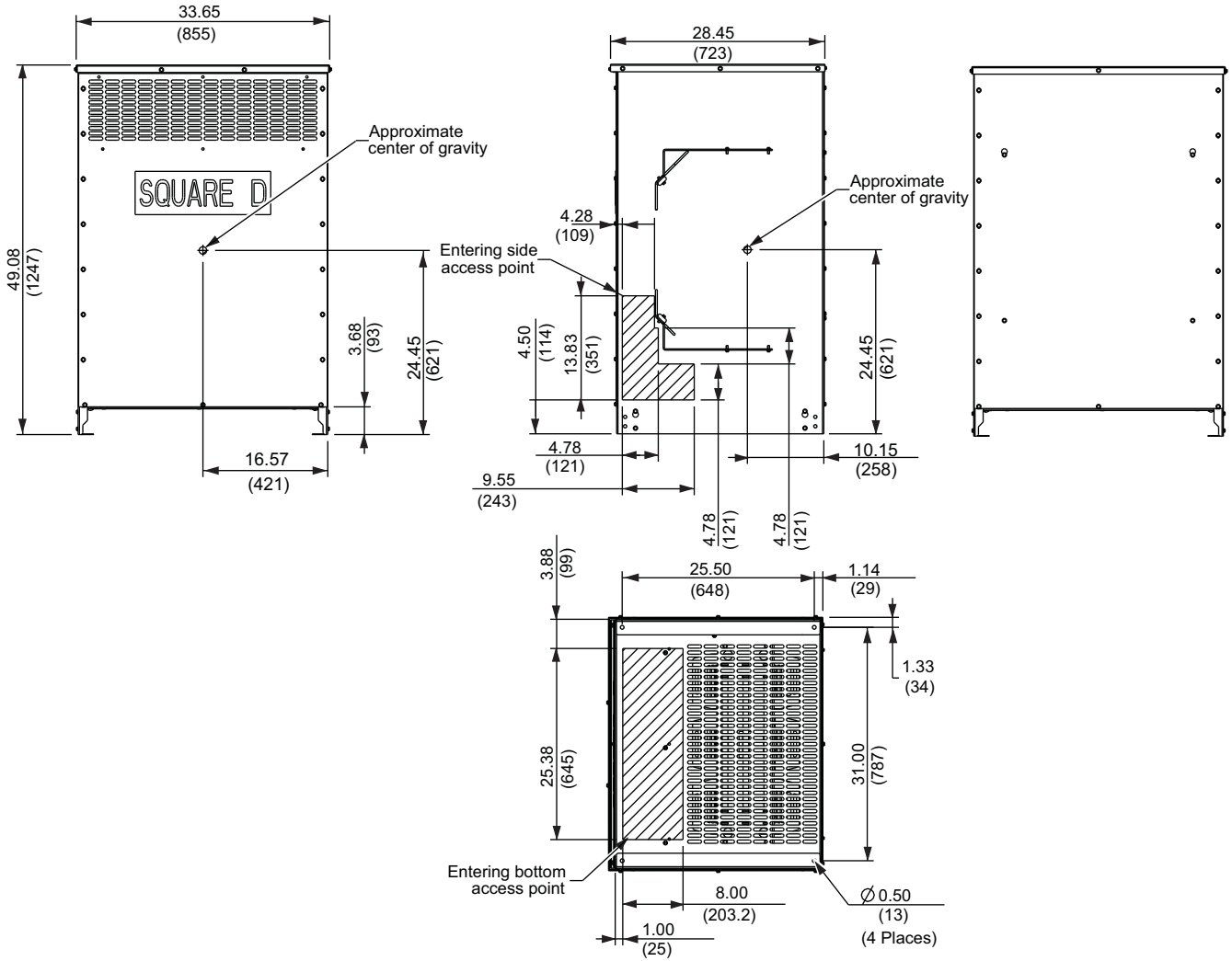
Figure 11: Enclosure 22K
