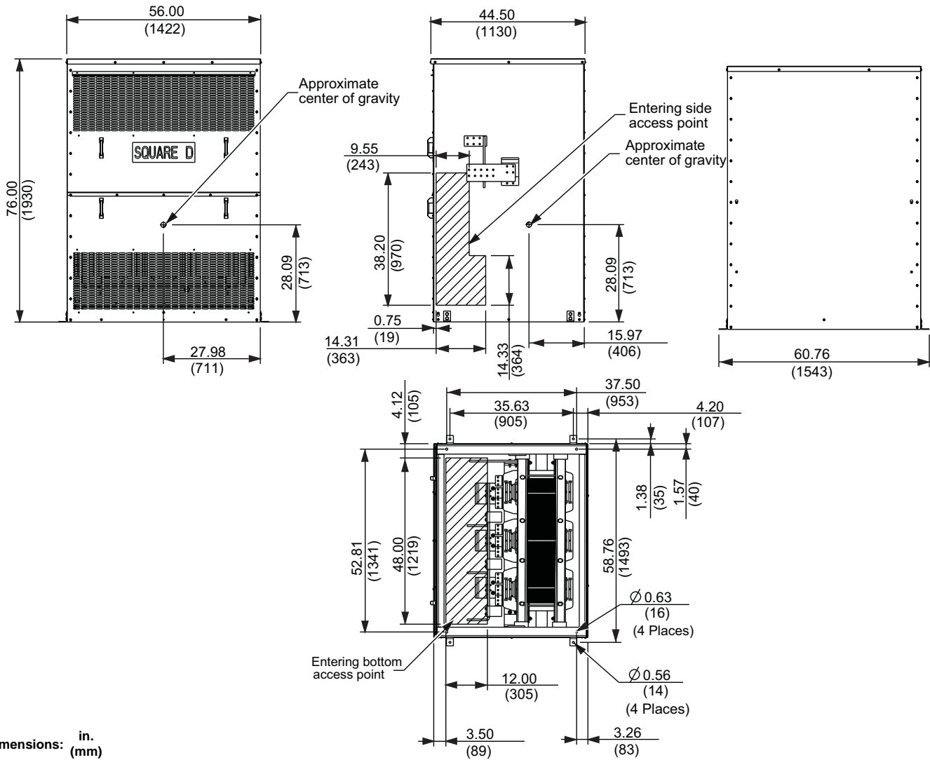
Figure 14: Enclosure 31J
