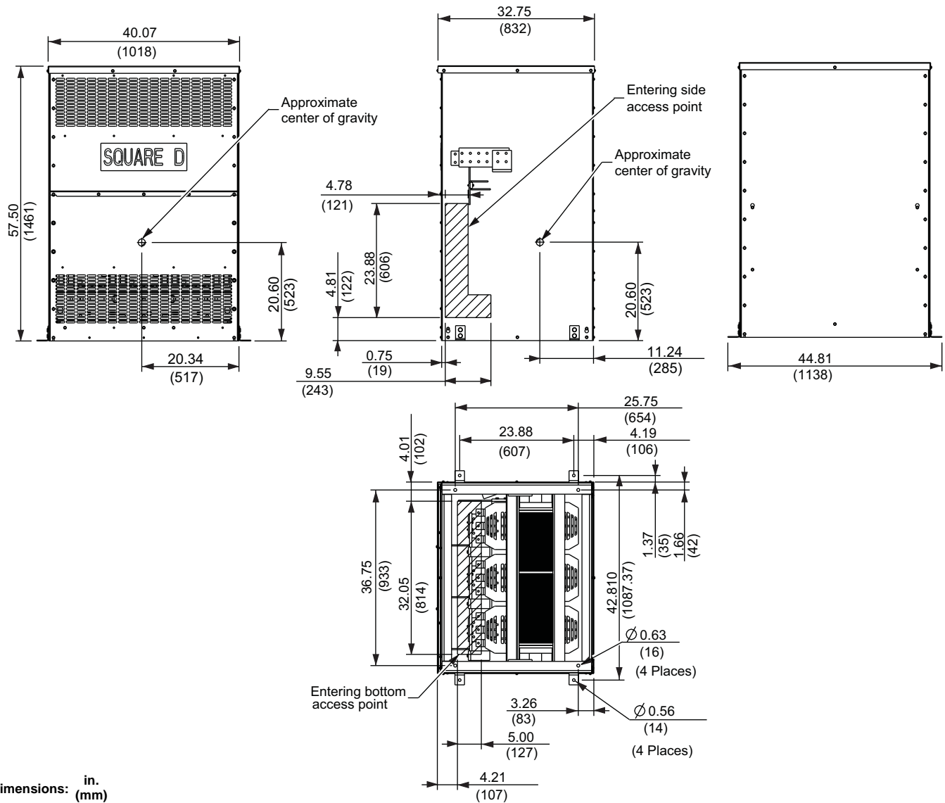
Figure 12: Enclosure 25J
