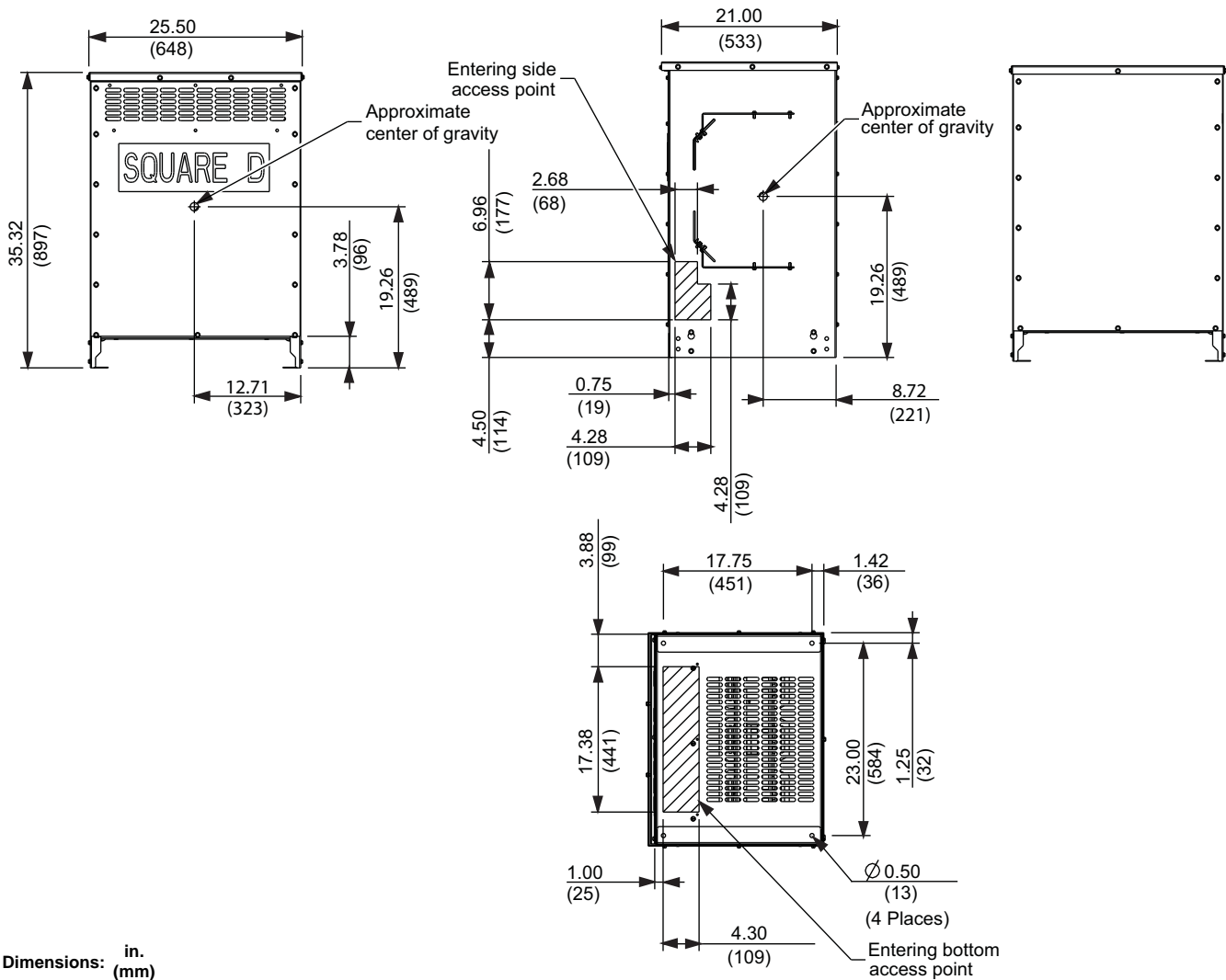
Figure 8: Enclosure 18K
