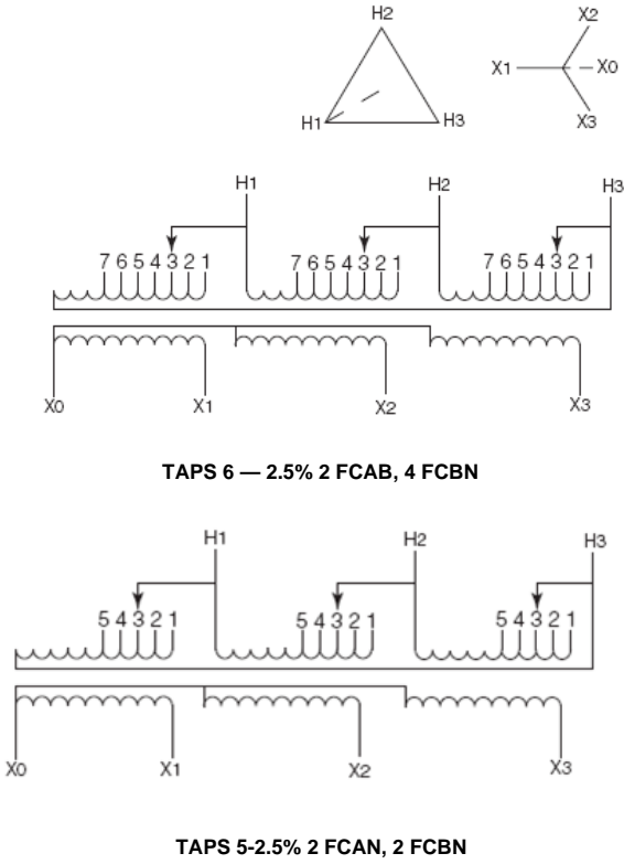
Figure 5: Phase Relationships / Wiring Diagram
