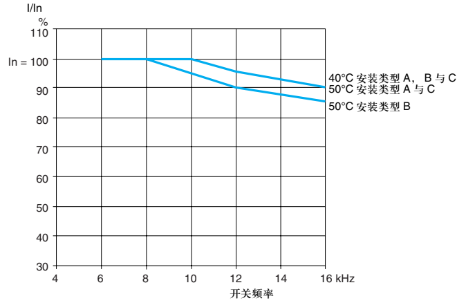
ATV 21HD30M3X
